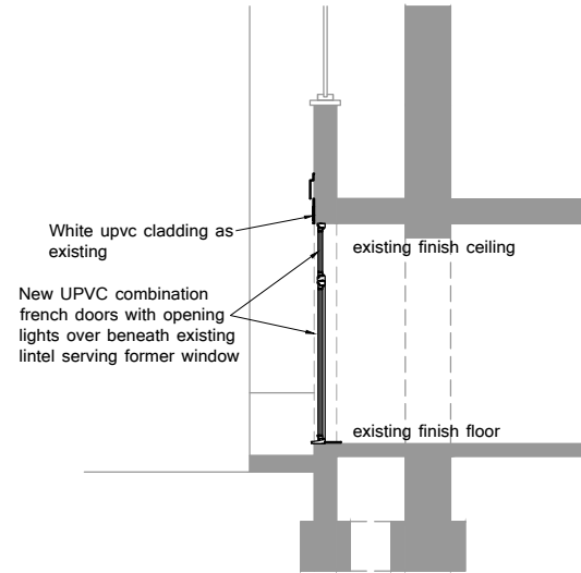
Proposed Section X-X
