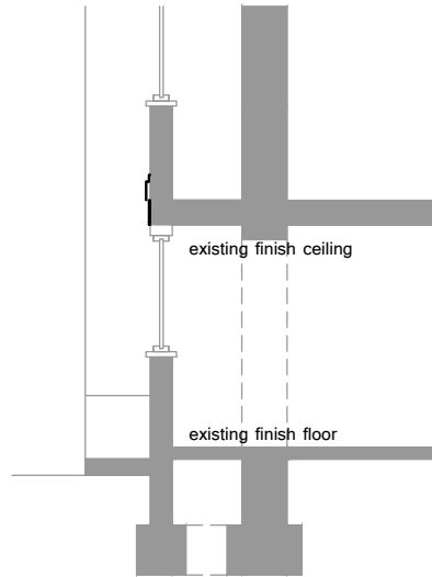
Existing Section X-X
