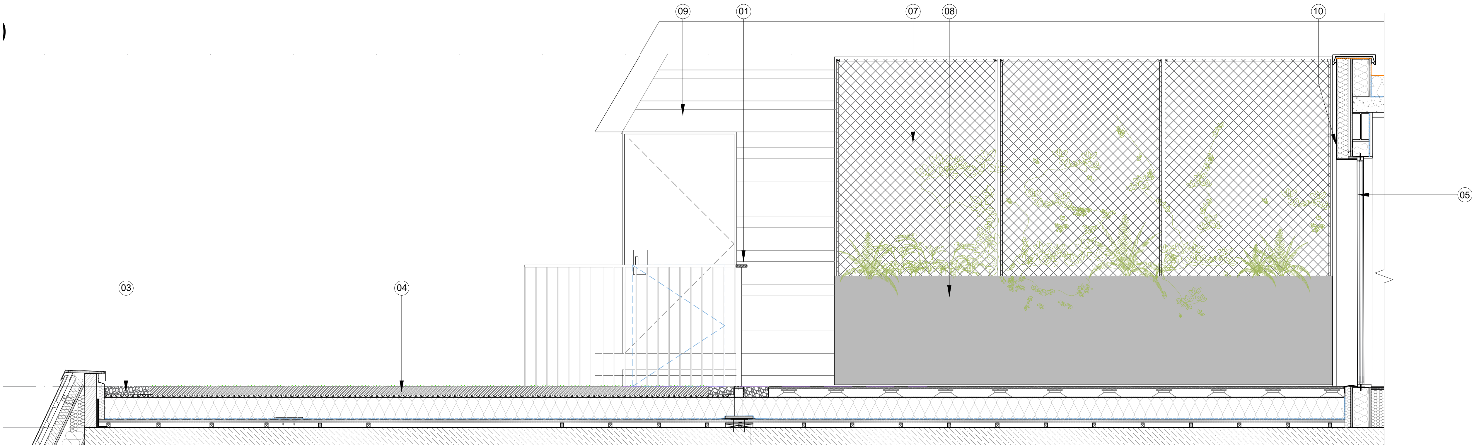
02 Terrace Elevation 2 30.608 1:20@A1,
