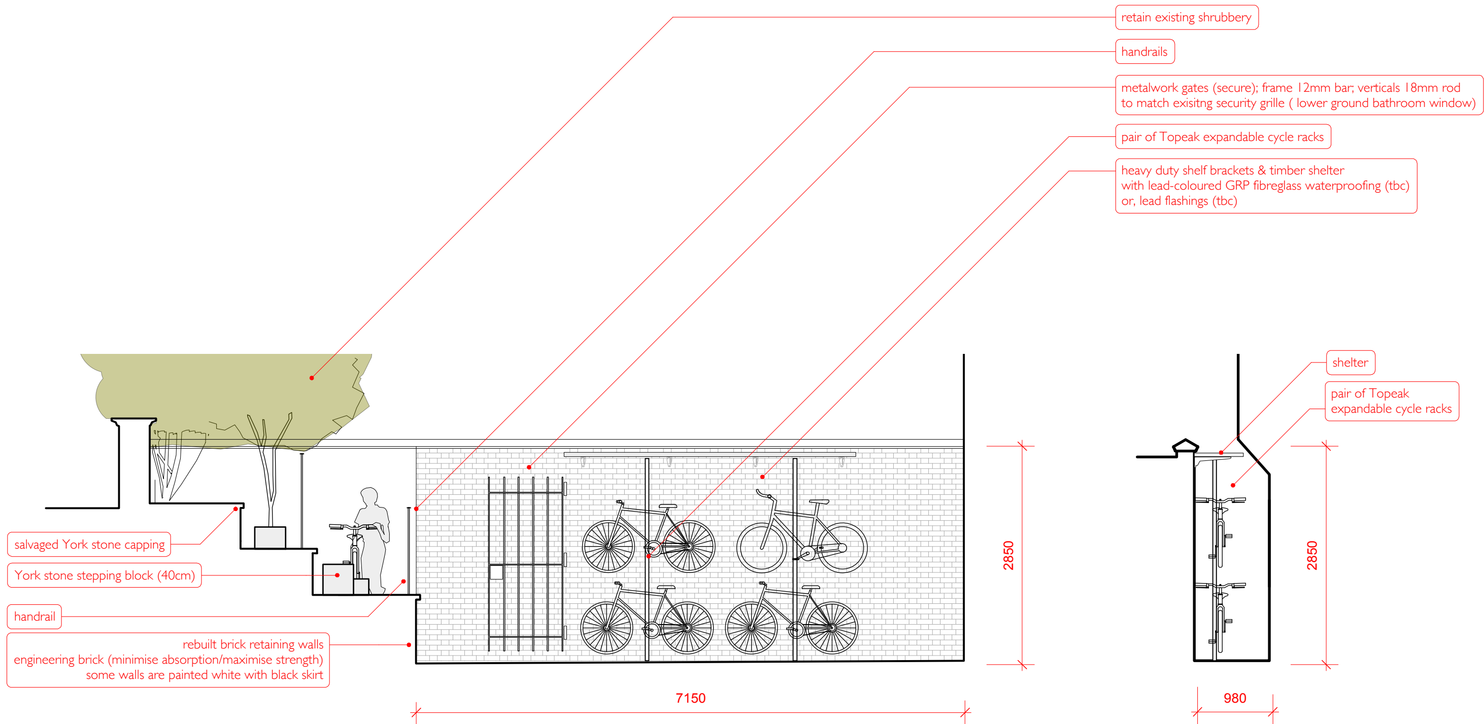
1 Terraced Garden & Secure Cycle Storage (side elevation) 1:50@ A3
