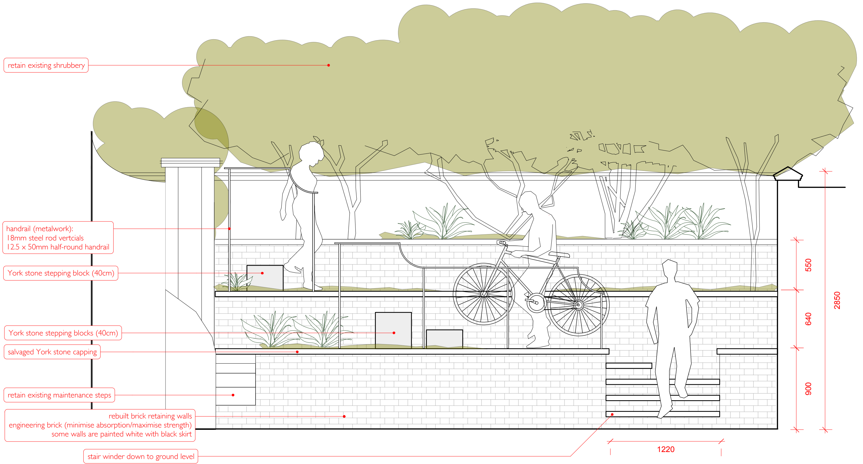
1 Terraced Garden (elevation) 1:25@ A3
