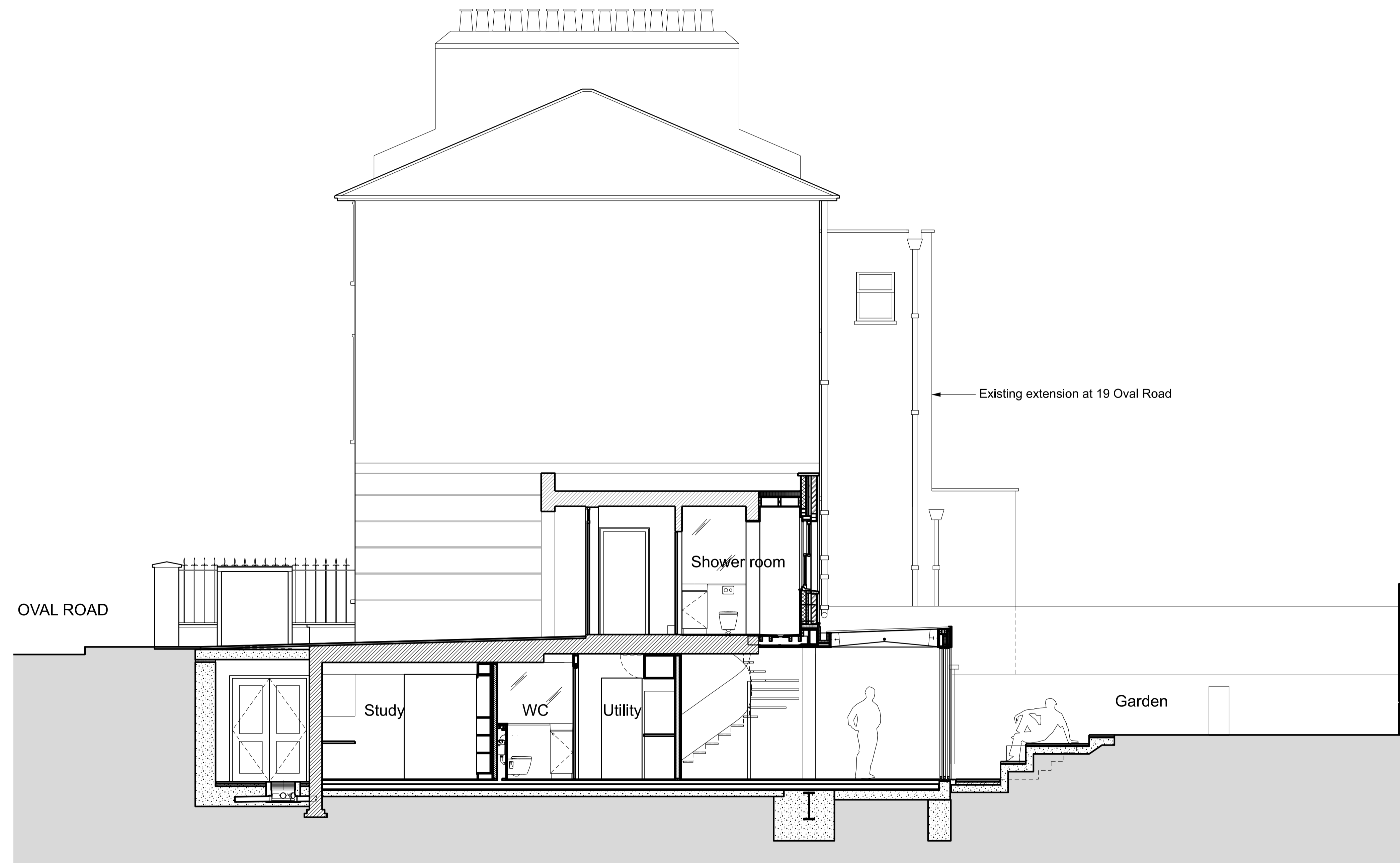
C Side Elevation
