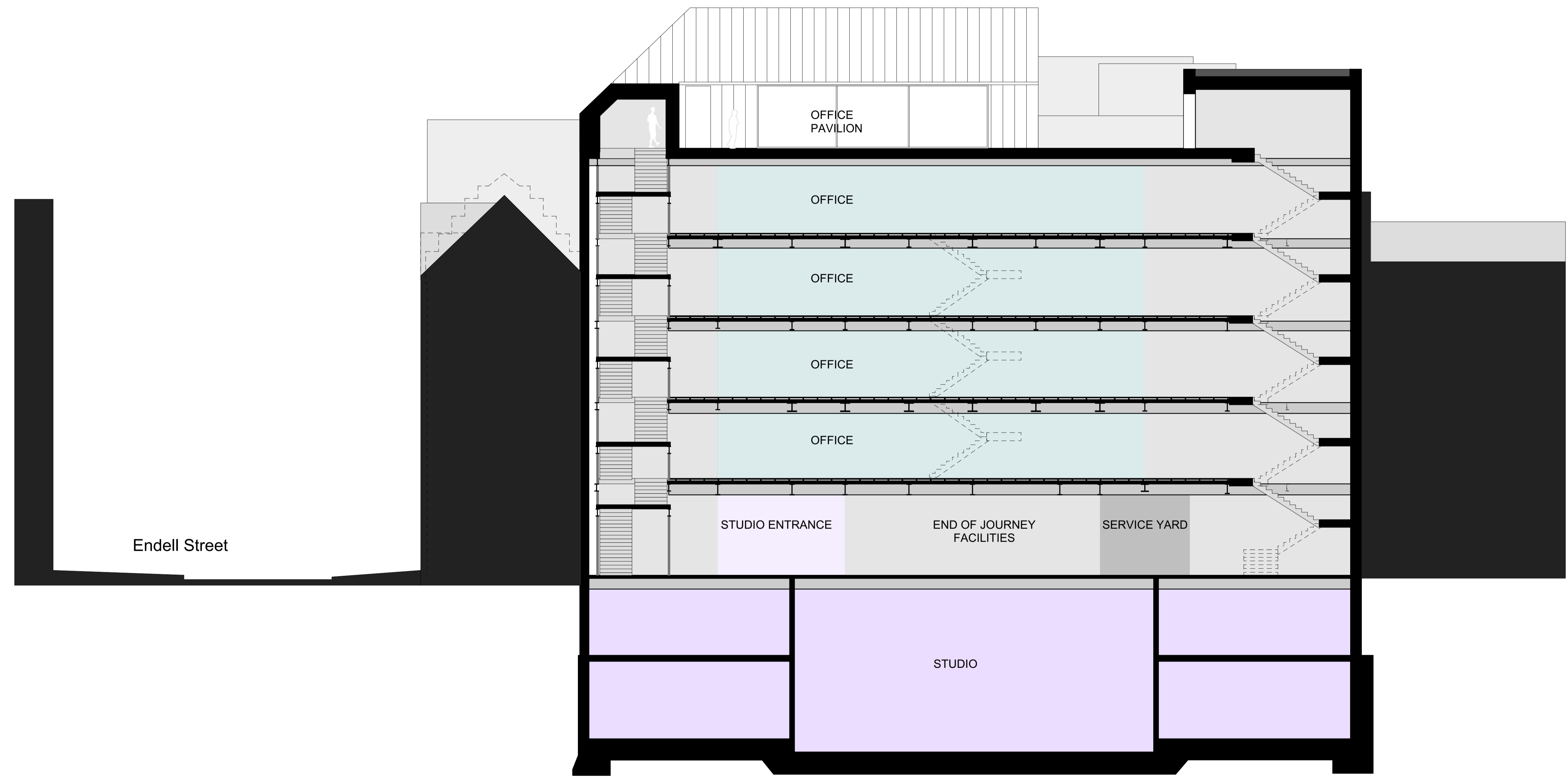
Proposed Section BB Scale: 1:100 NOTE: Any partitions omitted for clarity
