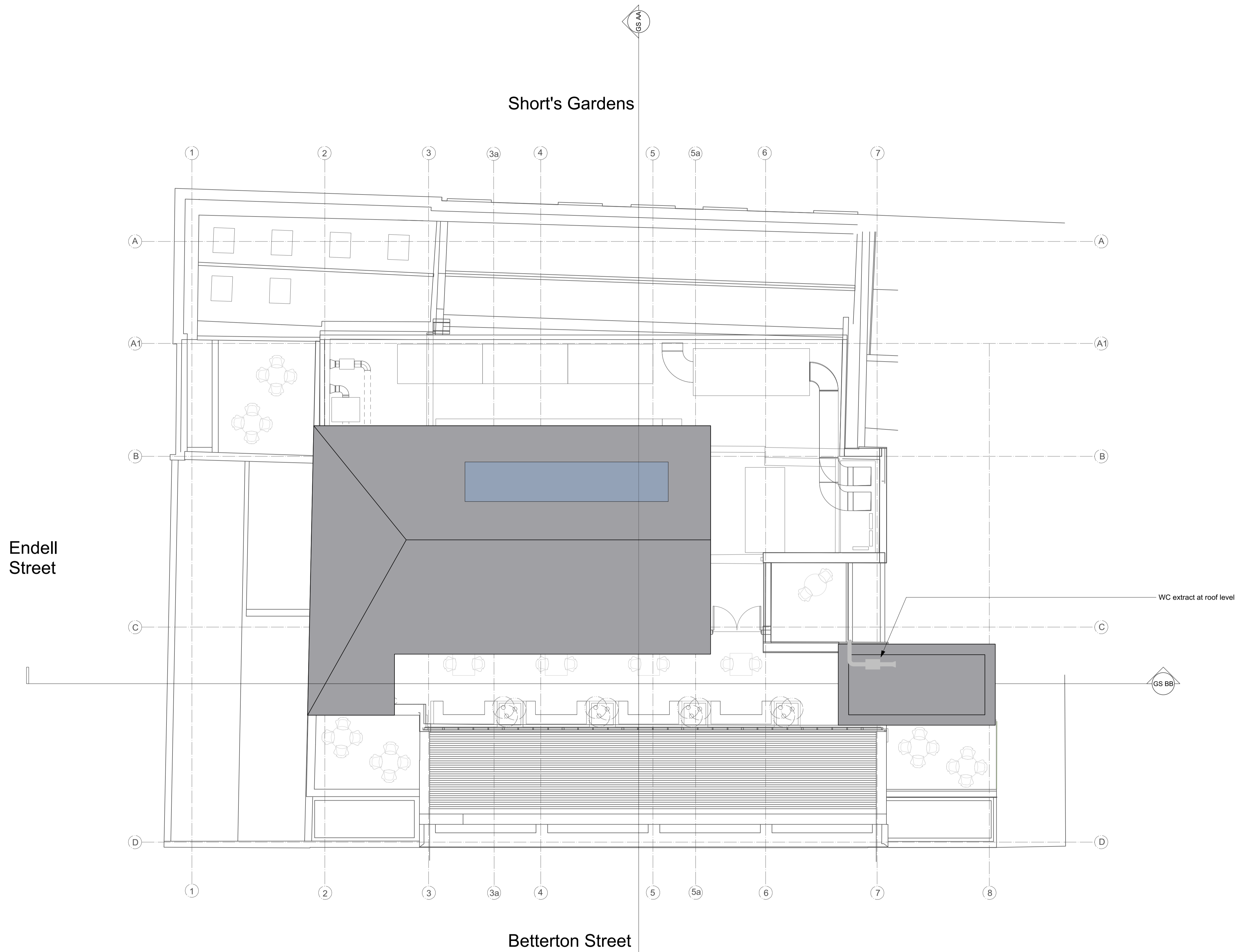
Roof Level Plan - Proposed Scale: 1:100
