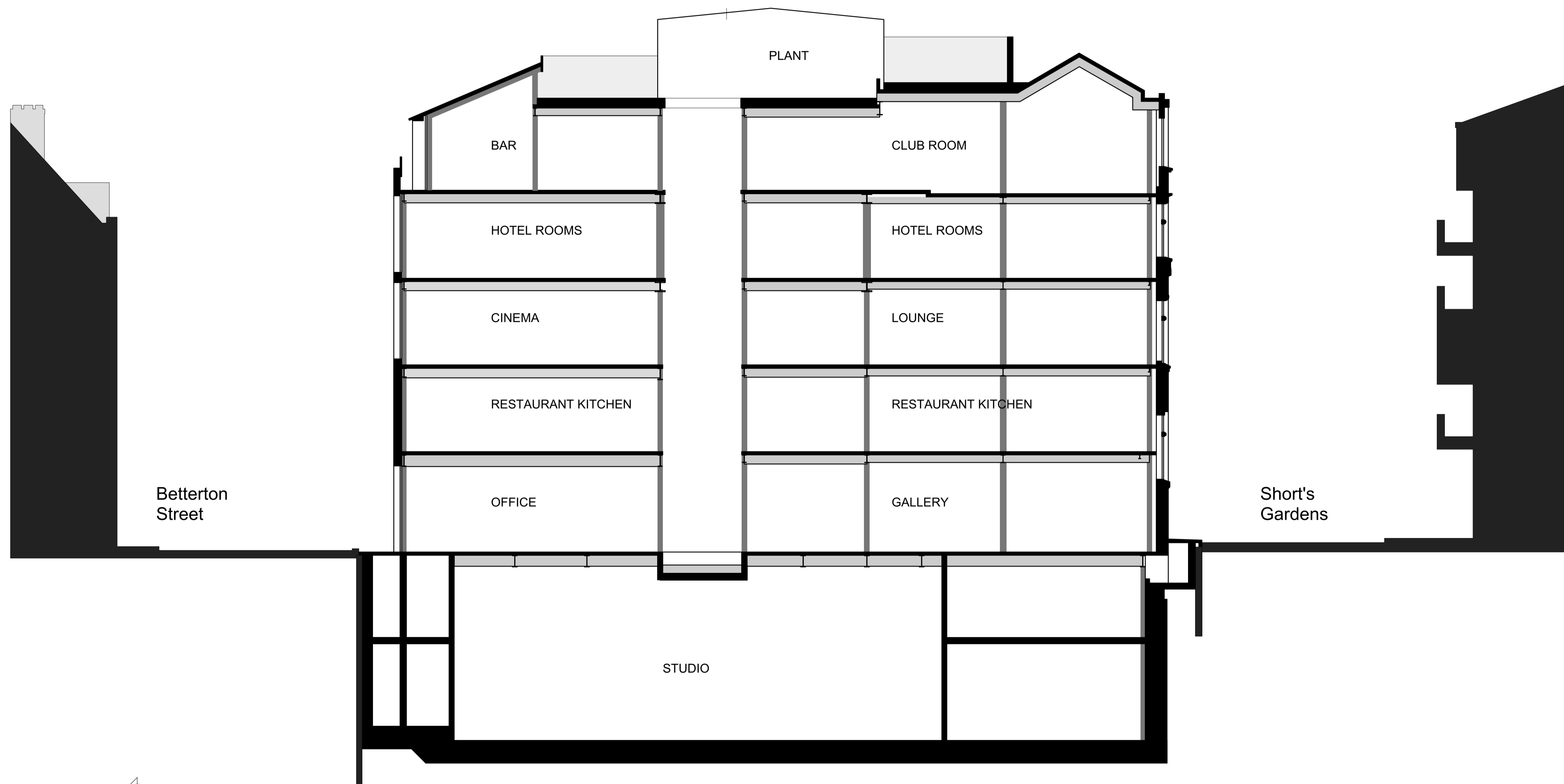
Existing Section AA Scale: 1:100 NOTE: Any partitions omitted for clarity
