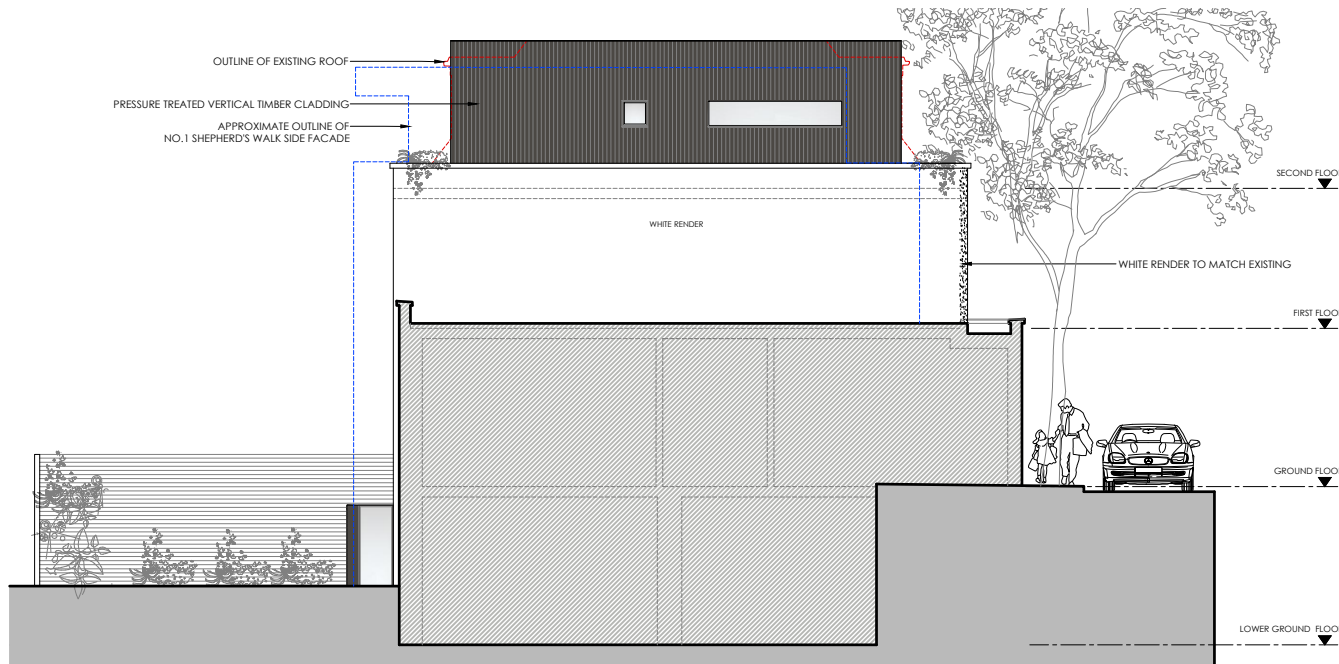
2 SIDE ELEVATION (VIEW FROM NO.1) PROPOSED (OPTION-B) 1:100
