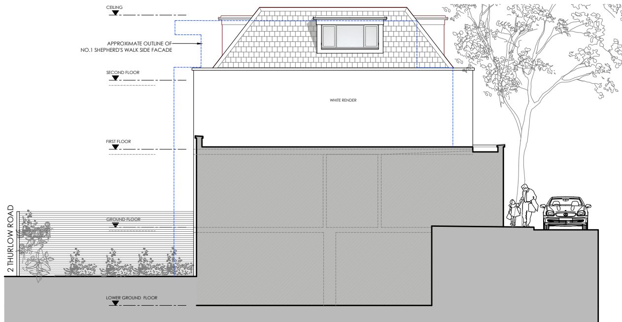
② SIDE ELEVATION (VIEW FROM NO.1) EXISTING 1:100
