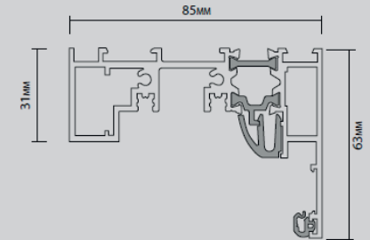
FRAME HEAD
