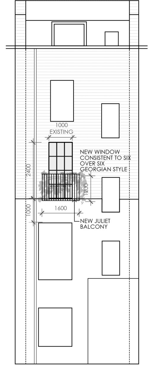
PROPOSED EAST ELEVATION (REAR OF TERRACE) SCALE 1:100
