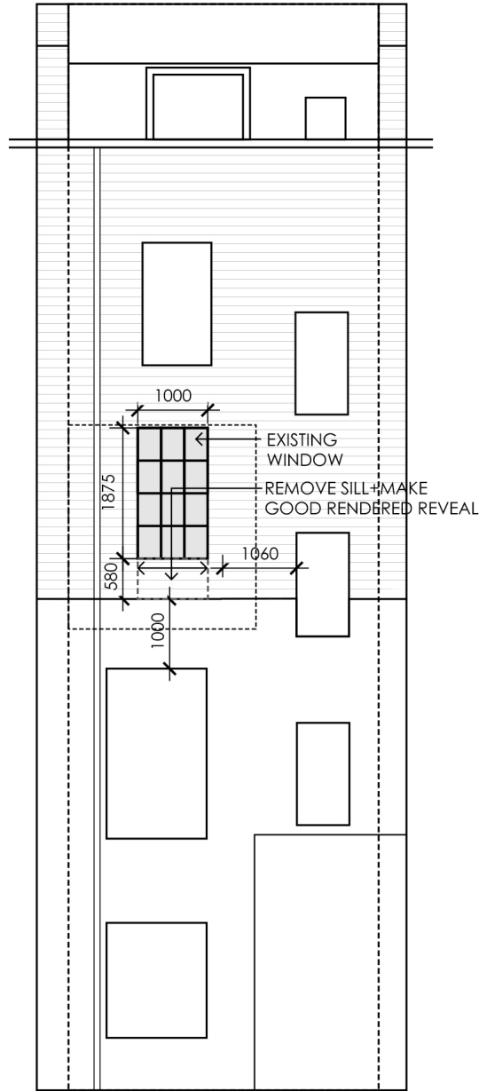
EXISTING EAST ELEVATION (REAR OF TERRACE) SCALE 1:100
