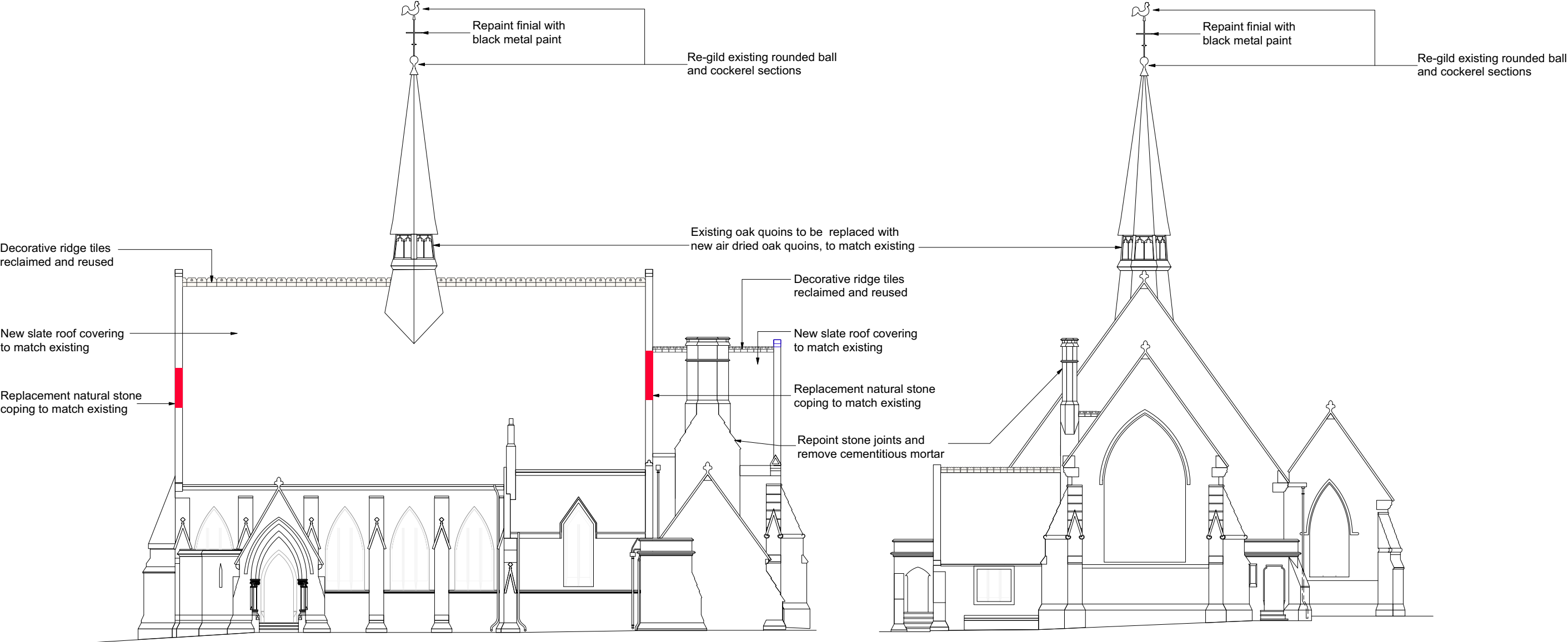
South Elevation
