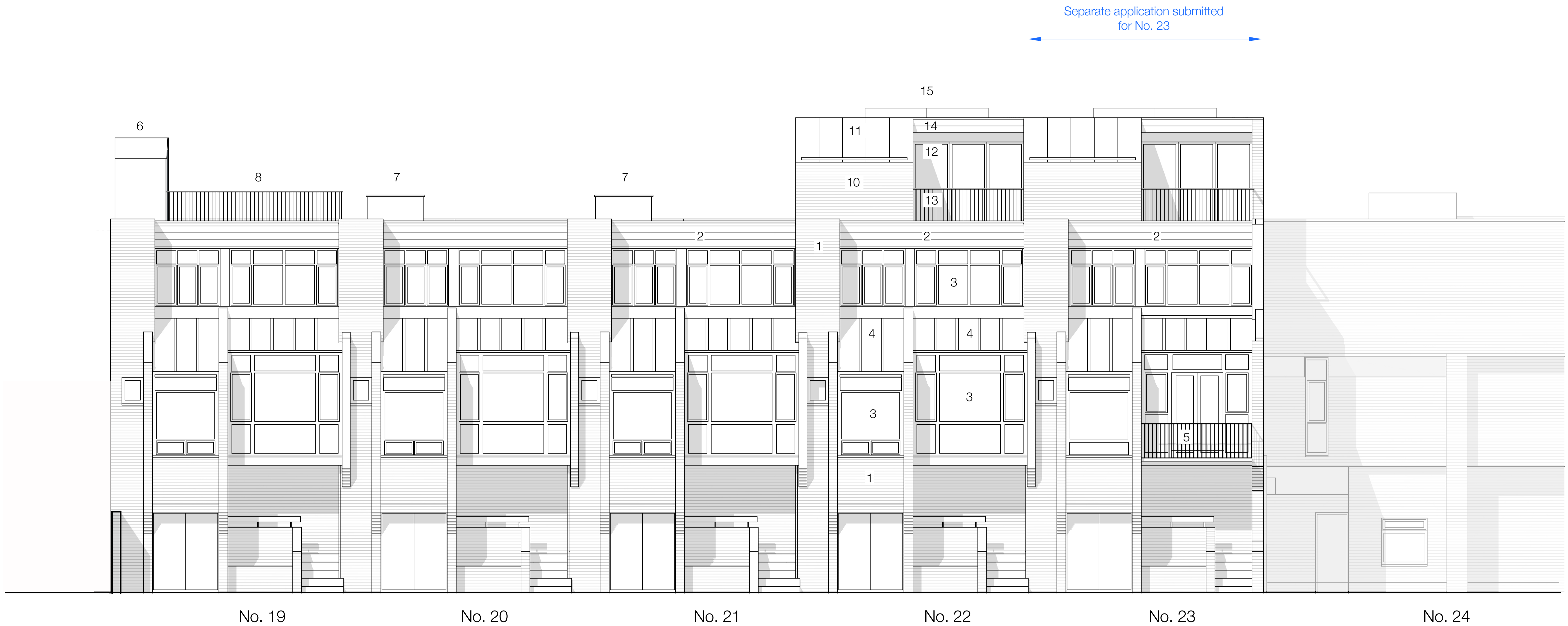
Proposed Elevation 1 (SE)
