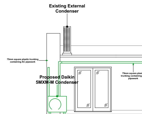
Courtyard Elevation 3
