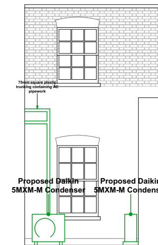
Courtyard Elevation 4
