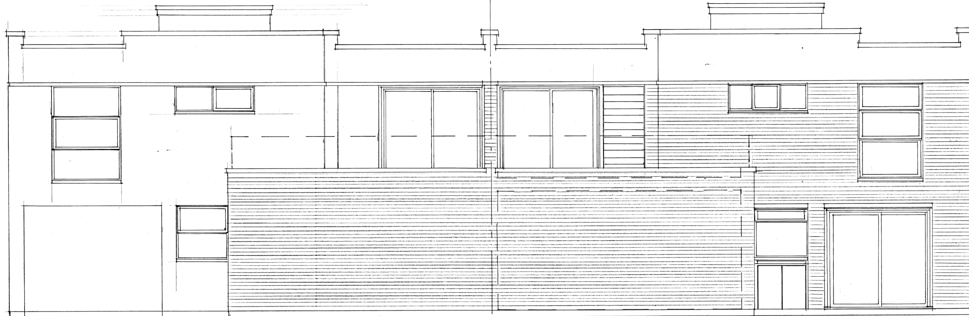
REAR ELEVATION
