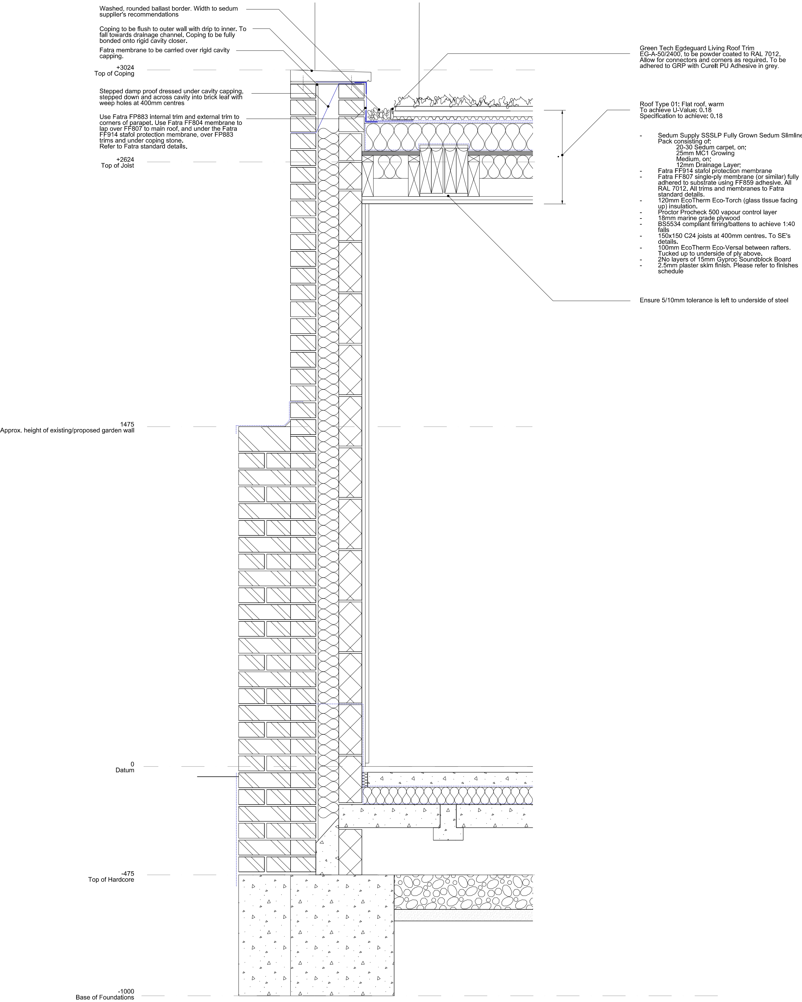
Detail 1: Sedum roof and parapet
