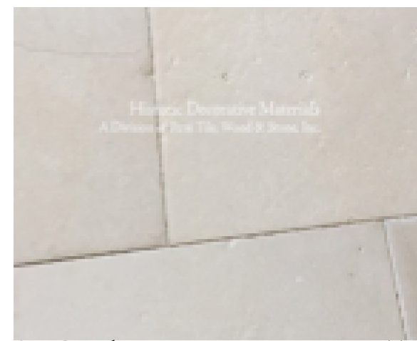
S1: Grey limestone
