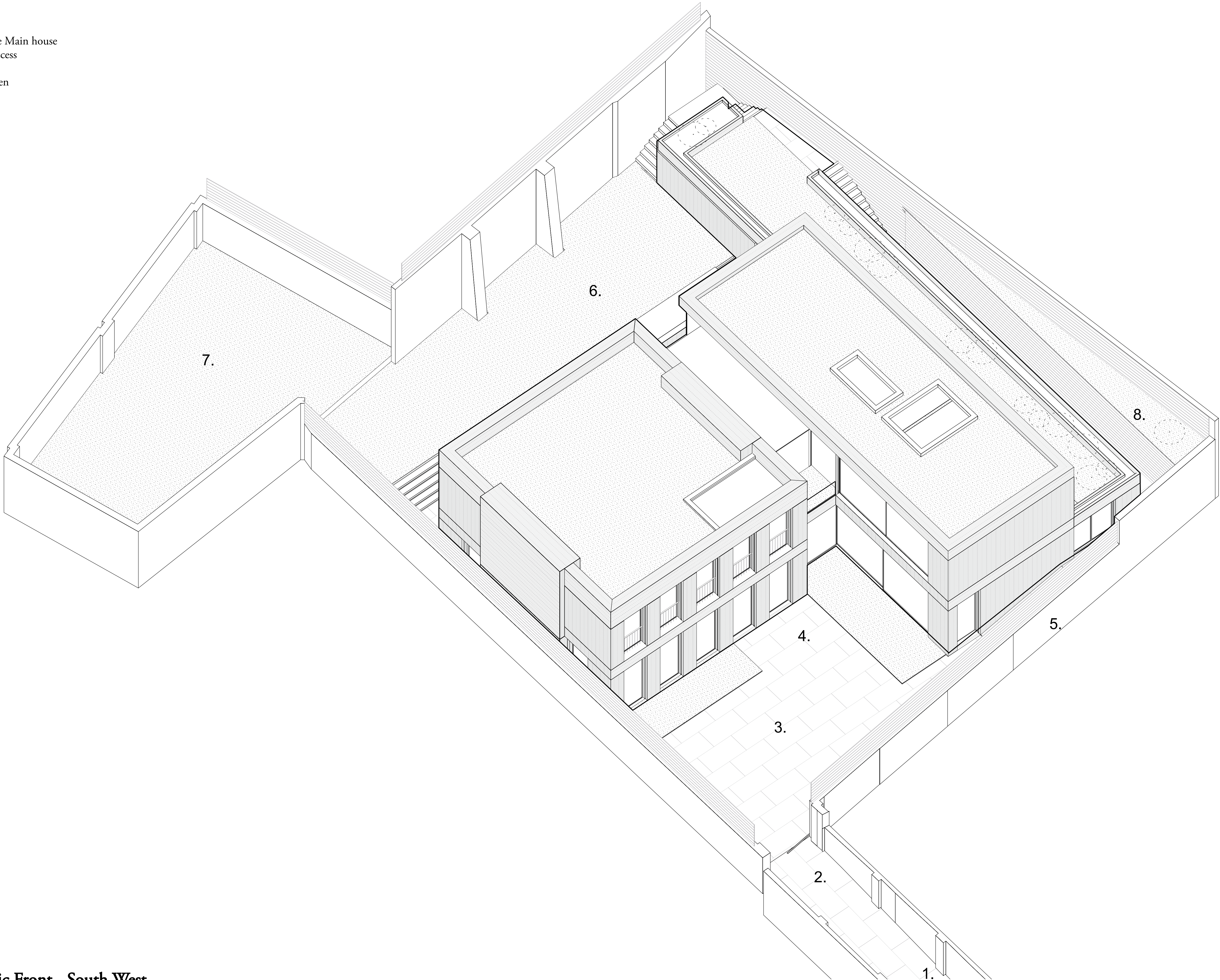
Axonometric Front - South West
