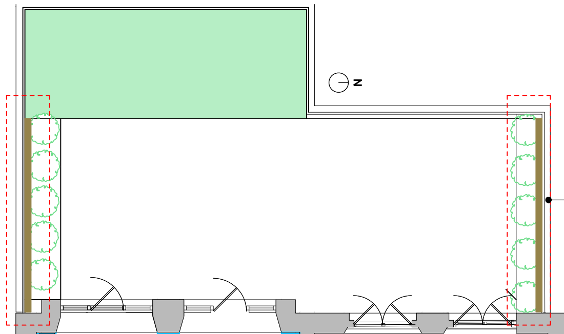
Proposed Screen Locations 1:75@A3
