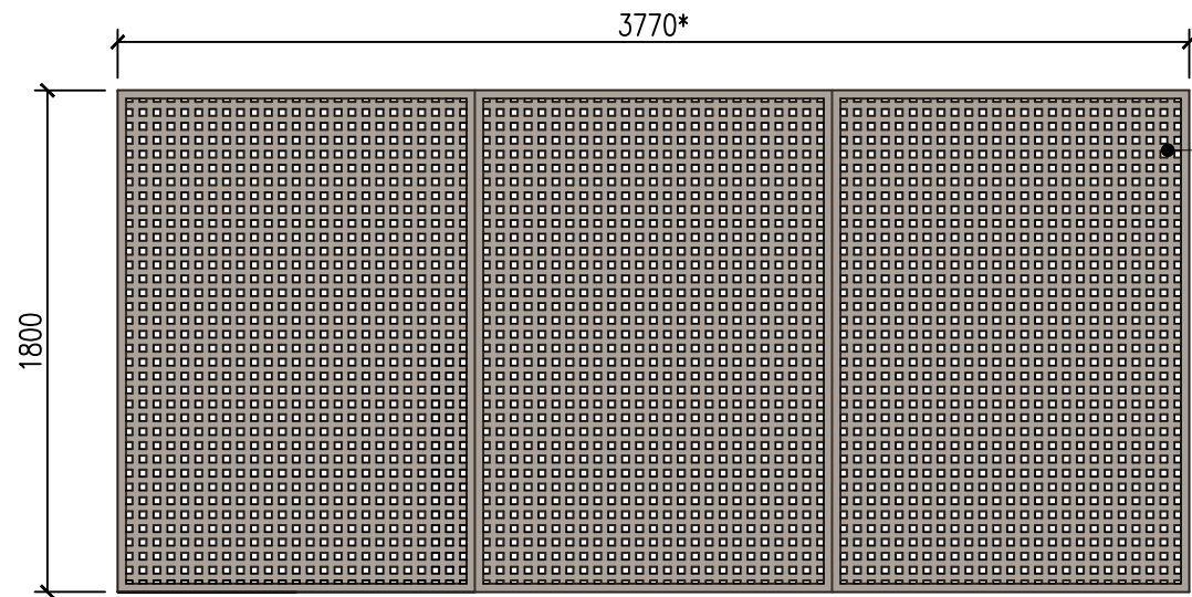
Proposed Screen Design 1:30@A3
