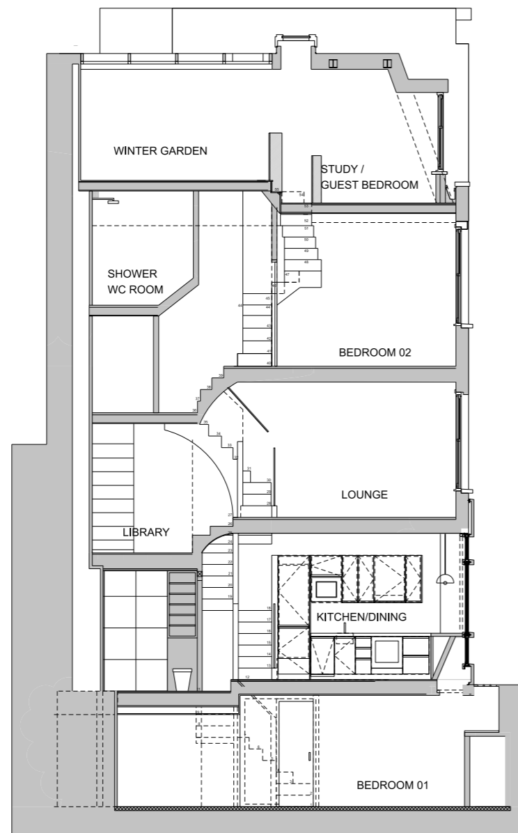
SECTION AA
