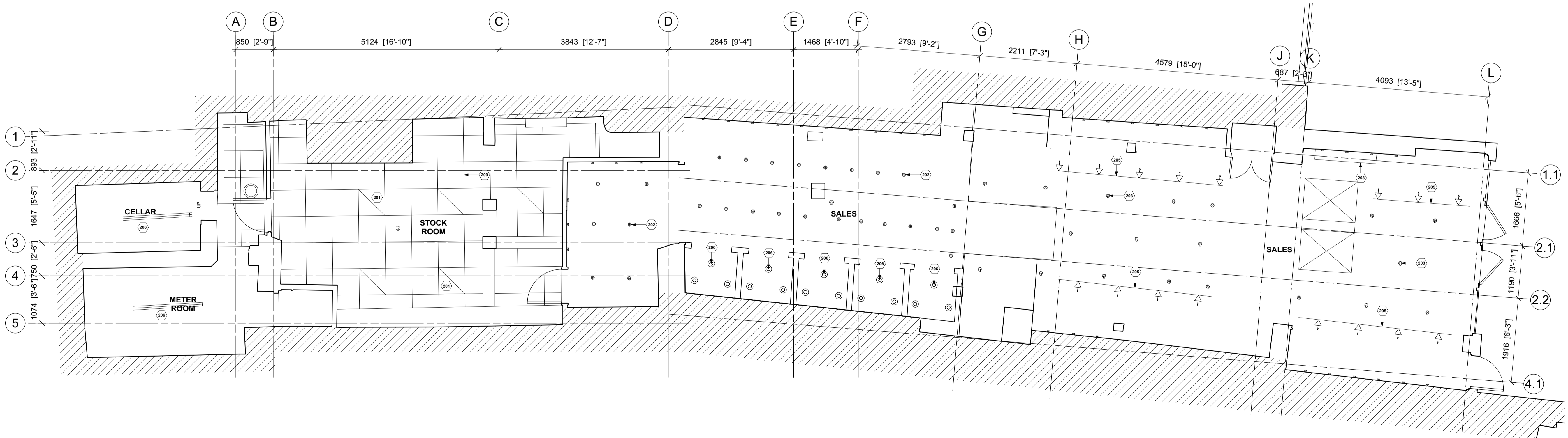
1 BASEMENT RCP PL200 SCALE: @A1 1:50
