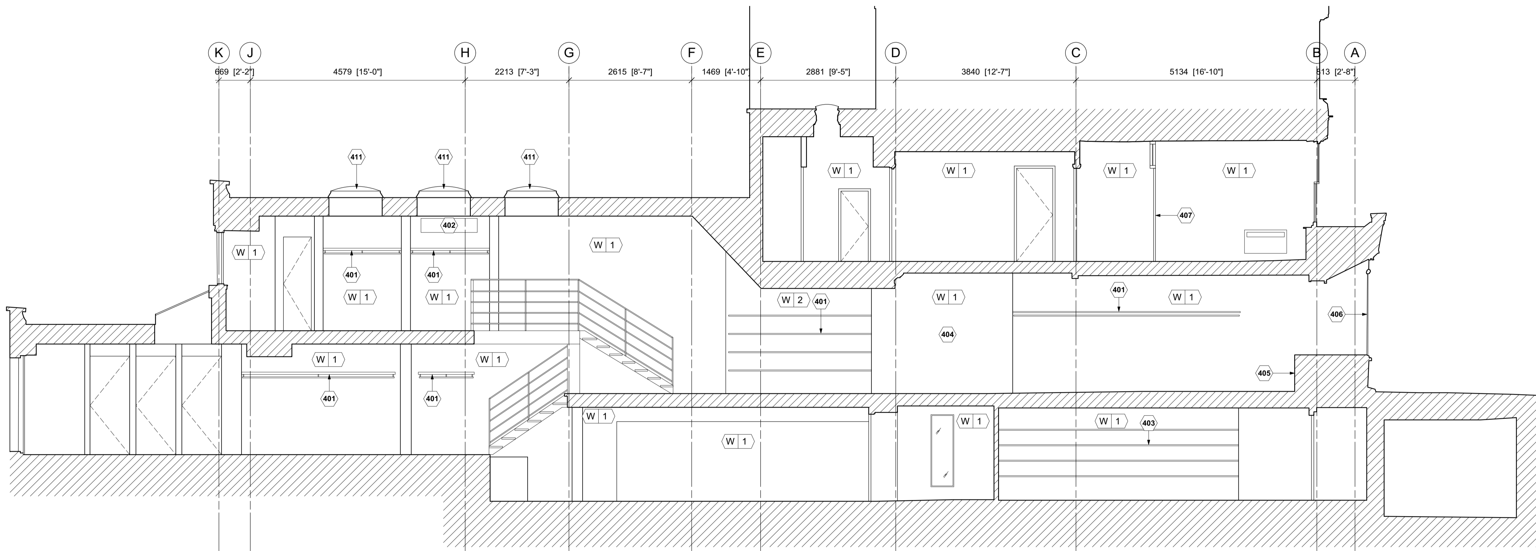
1 EXISTING SECTION 01 EX400 SCALE: @A1 1:50
