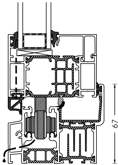
Option 1, Open Out Weathered track
