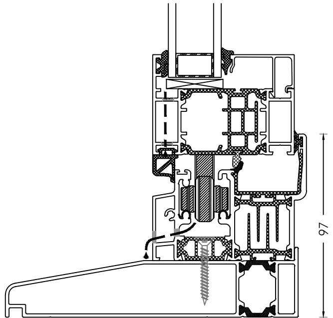
Option 3, Open Out Weathered track on Thermally Broken Sill
