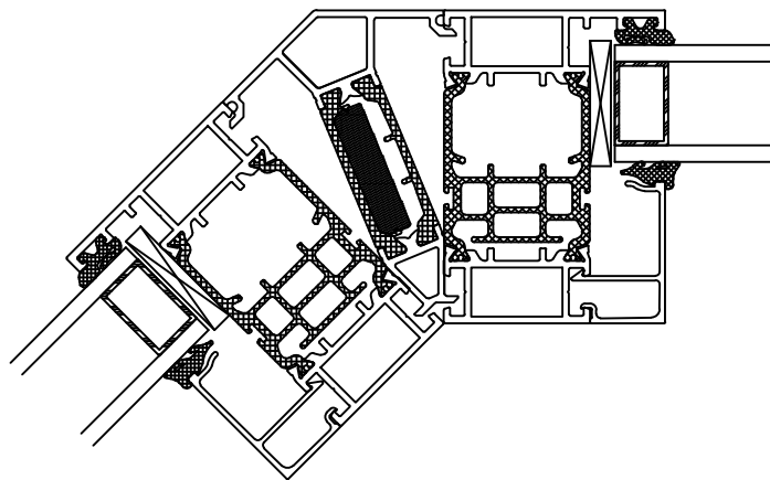
Fixed 135° Post with Fixed Panels
