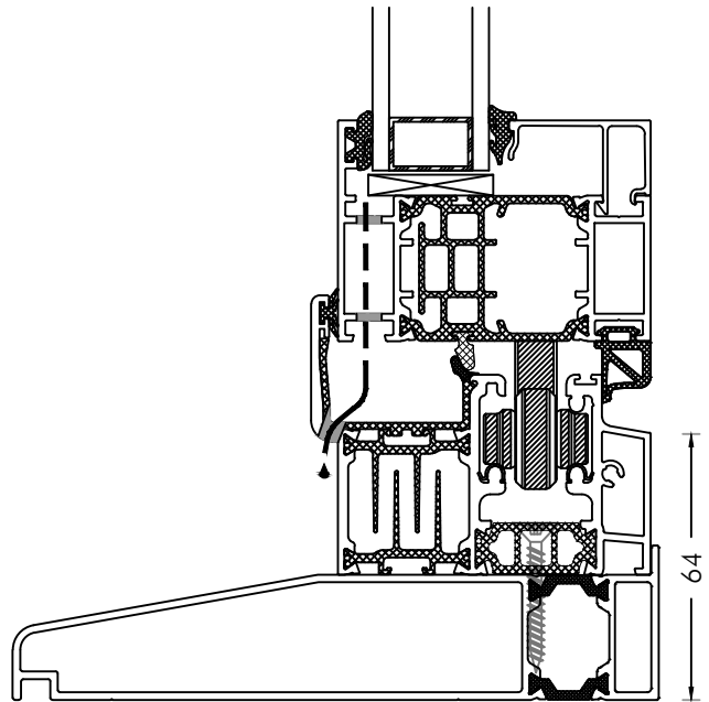
Option 4, Open In Weathered track on Thermally Broken Sill
