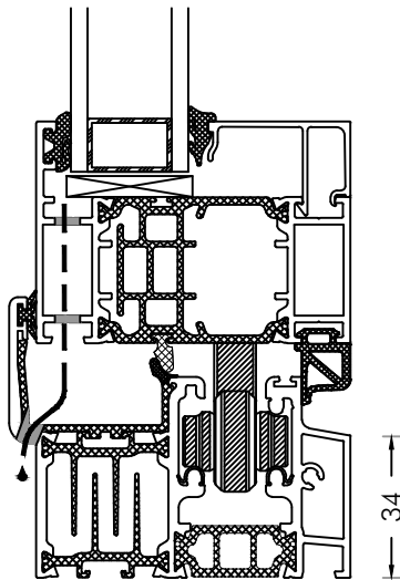
Option 2, Open In Weathered track
