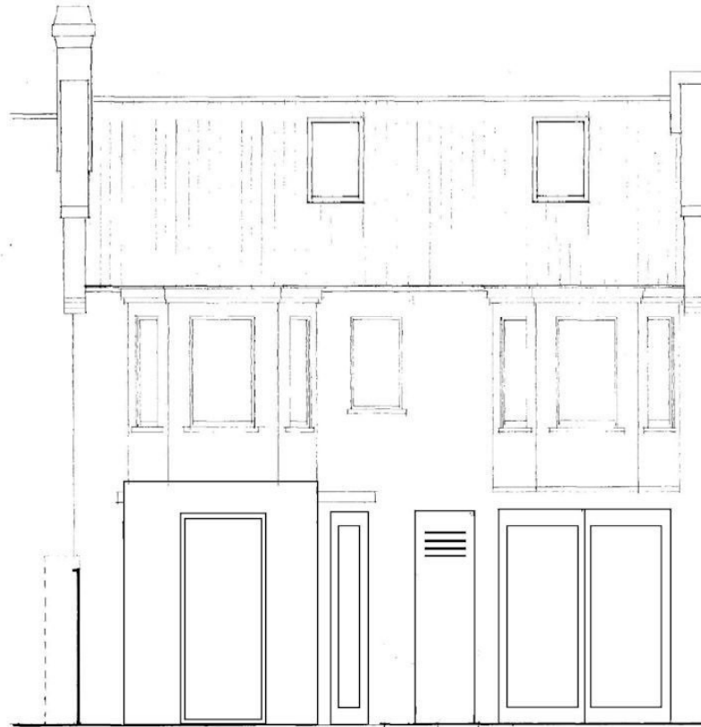
1 Lambolle Place Front view of ground floor windows/doors existing
