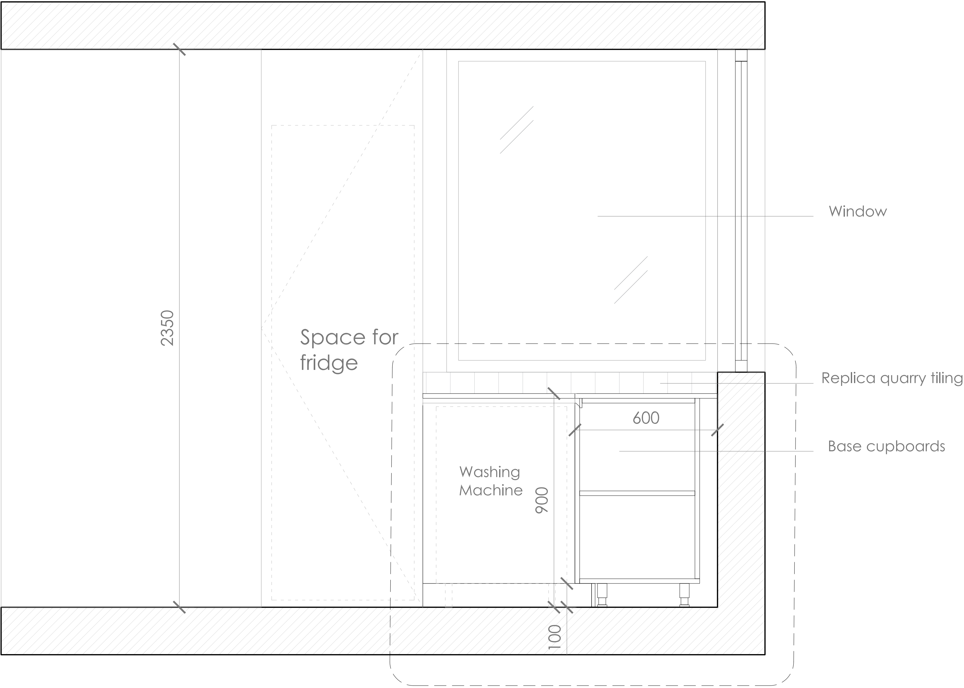
Detail Section 04 Scale 1:5
