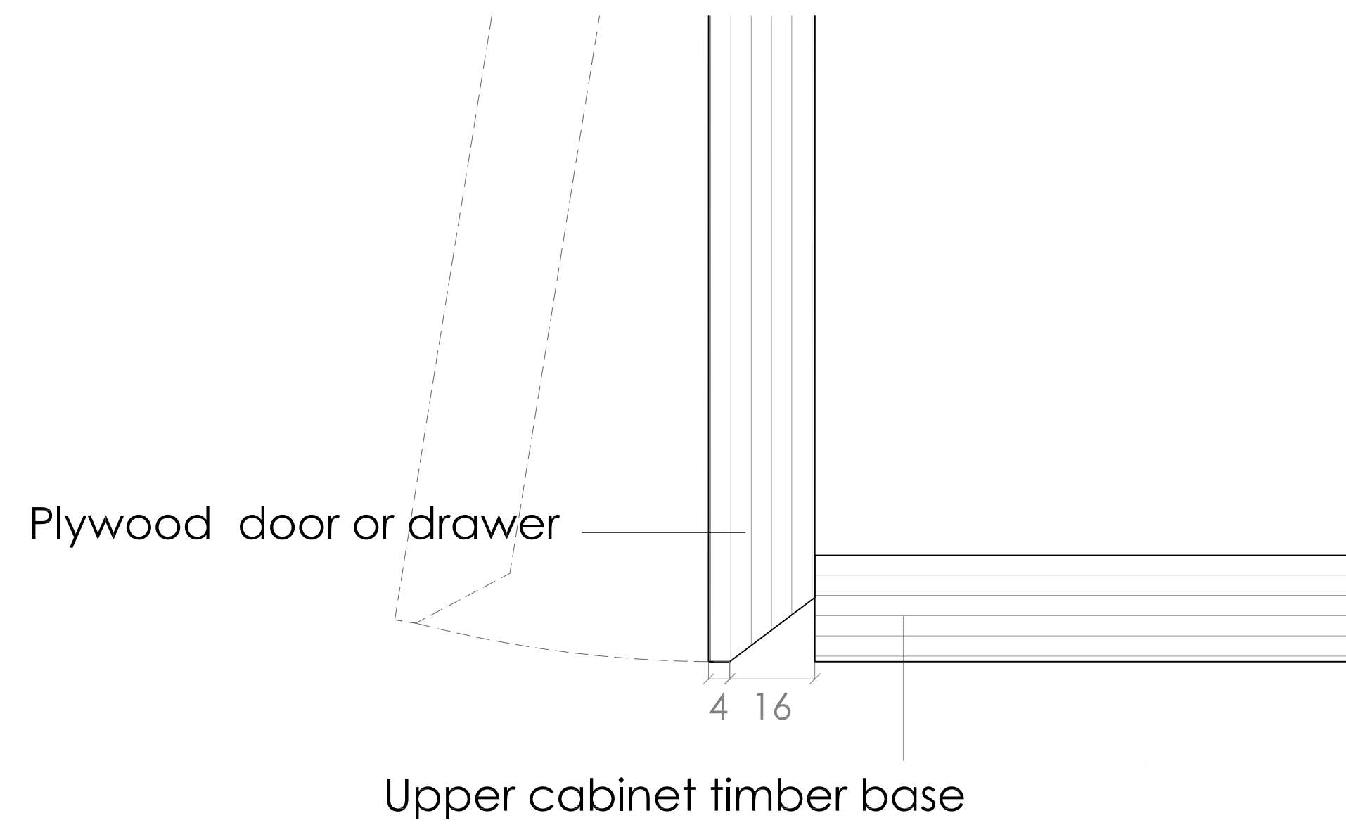
Detail 01 Scale 1:1
