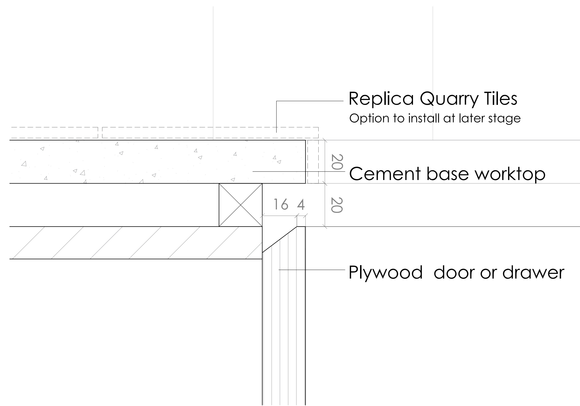
Detail 01 Scale 1:1
