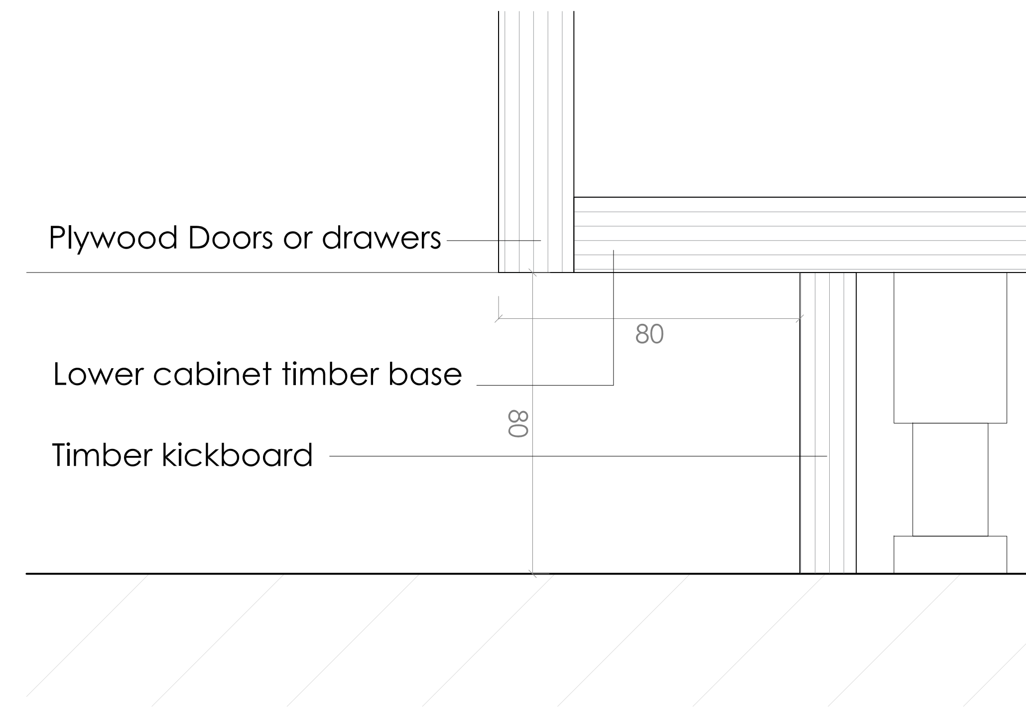
Detail 02 Scale 1:1
