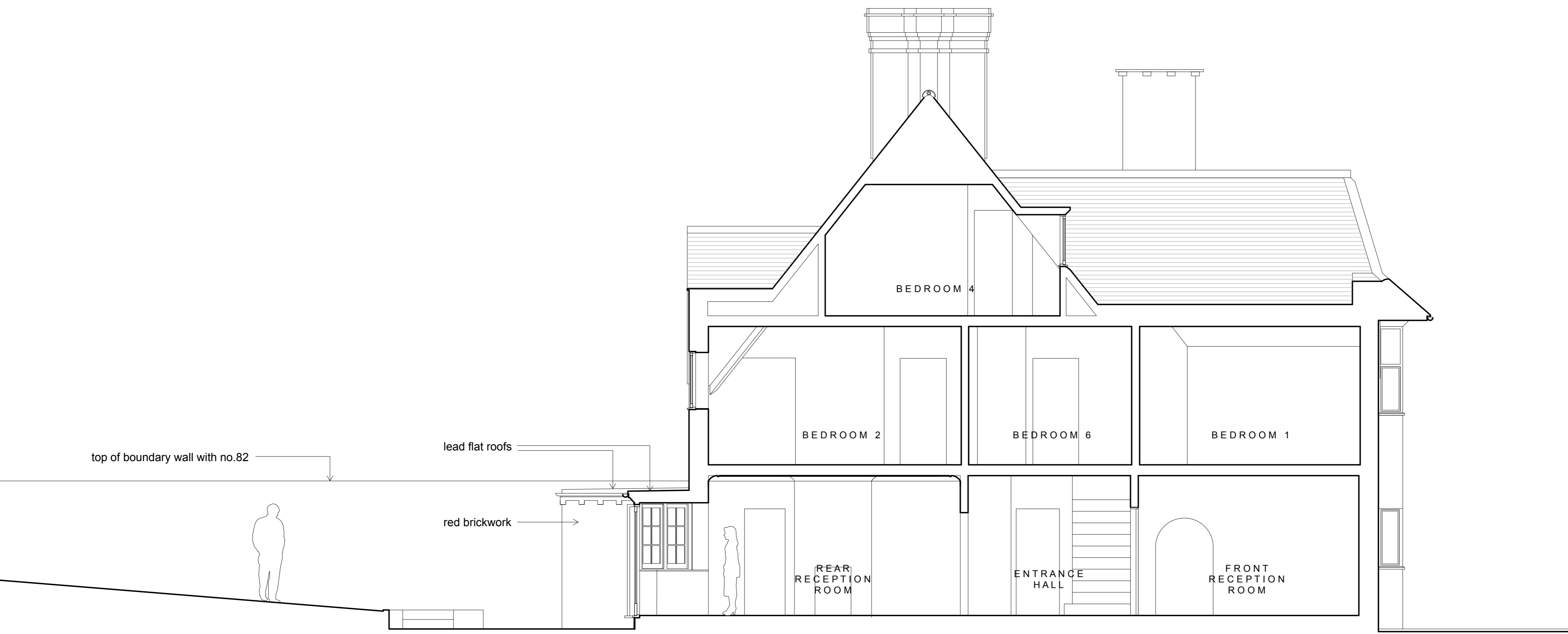
SECTION A-A AS EXISTING
