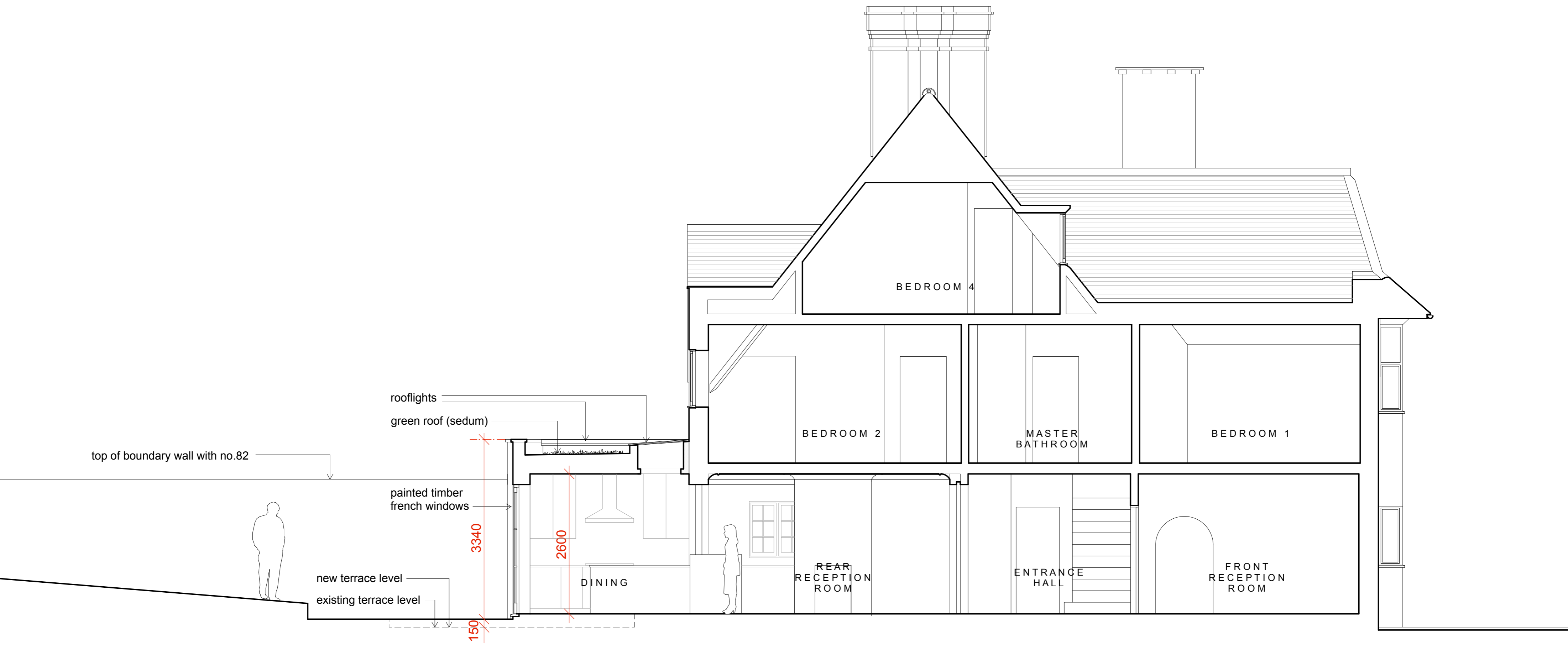
SECTION A-A AS PROPOSED
