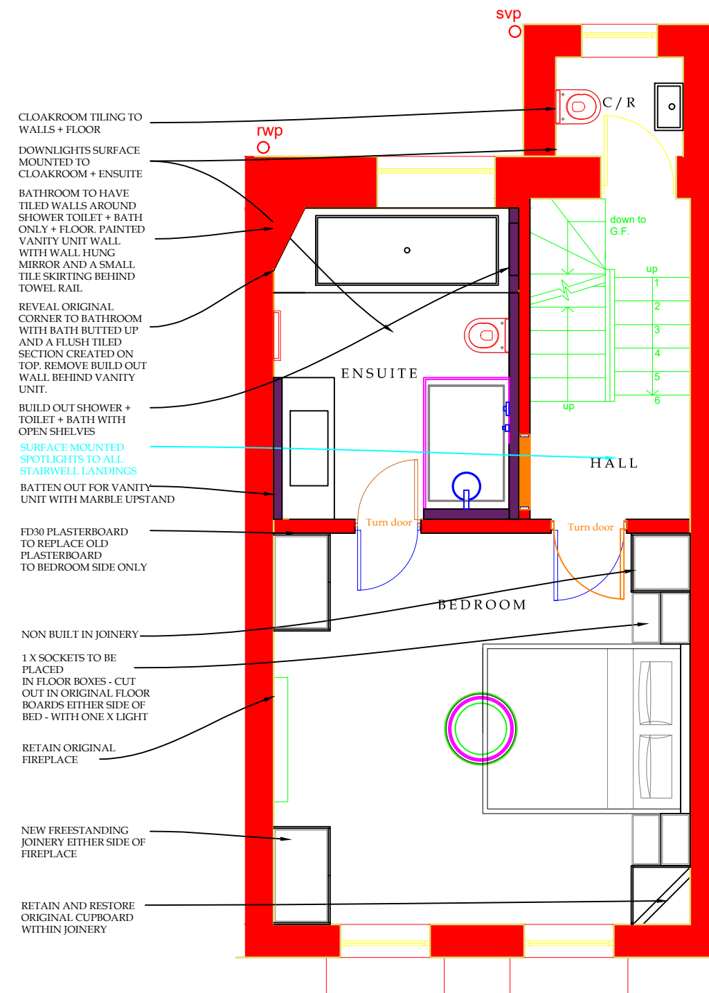
FIRST FLOOR
