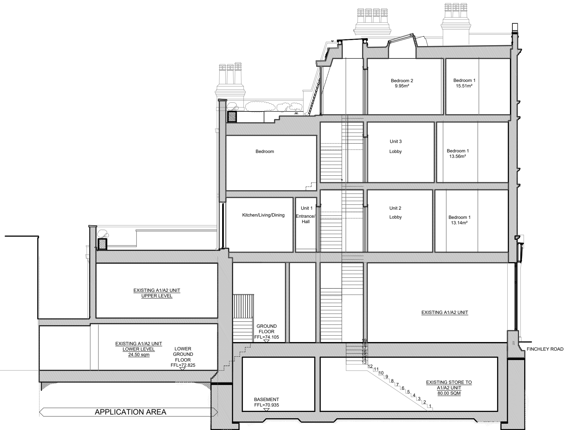
1 101 Section A-A Existing SCALE 1:100 @ A3
