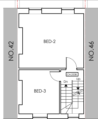
GIA-34.7m² ⊕ SECOND FLOOR PLAN EXISTING 1:100
