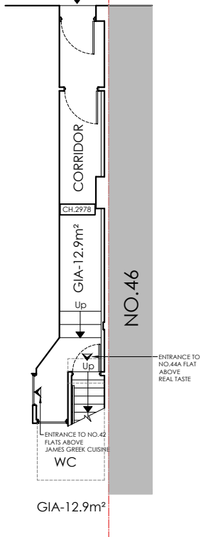
⊕ PARTIAL GROUND FLOOR PLAN EXISTING 1:100
