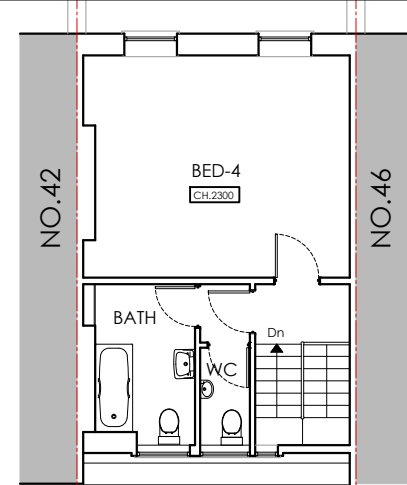
GIA-34.0m² ⊕ THIRD FLOOR PLAN EXISTING 1:100
