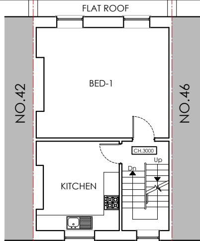
GIA-34.7m² FLAT ROOF SERVICE AREA ⊕ FIRST FLOOR PLAN EXISTING 1:100
