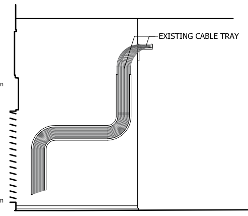
E2 ELEVATION E4 - RETURN WALL AS EXISTING 1:50@A1
