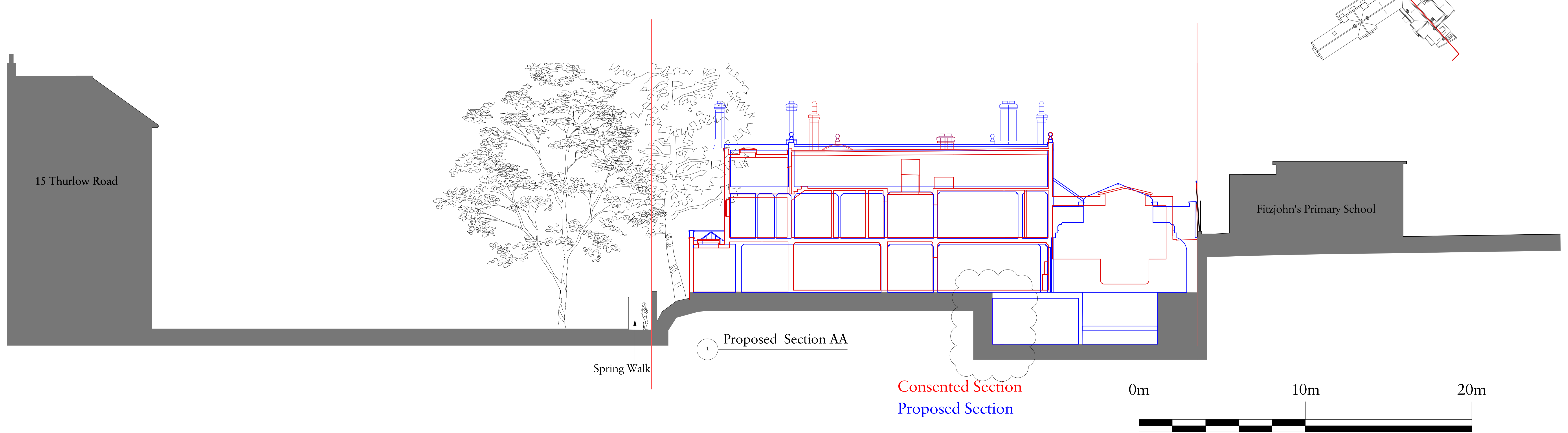
Proposed Section AA
