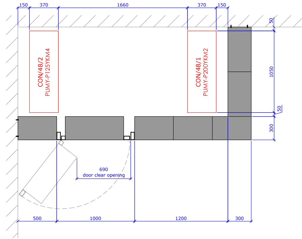
Plan (without roof)
