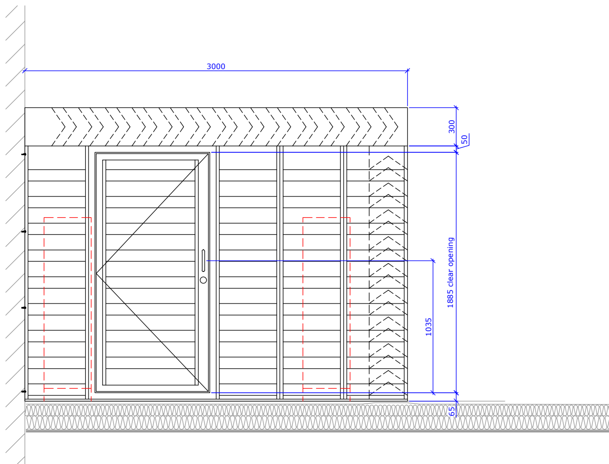
East Elevation
