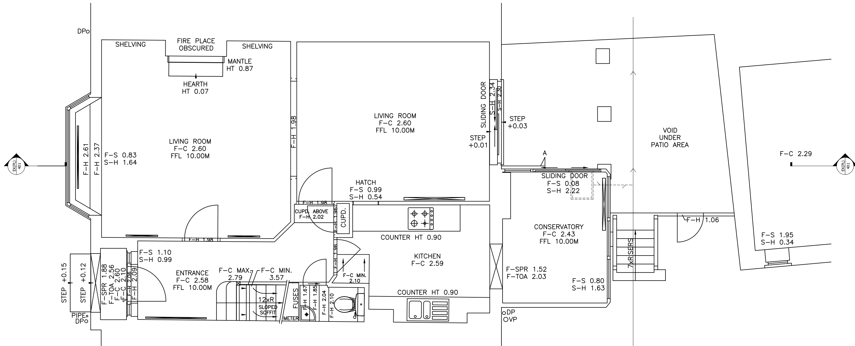
01 Existing Ground Floor Plan
