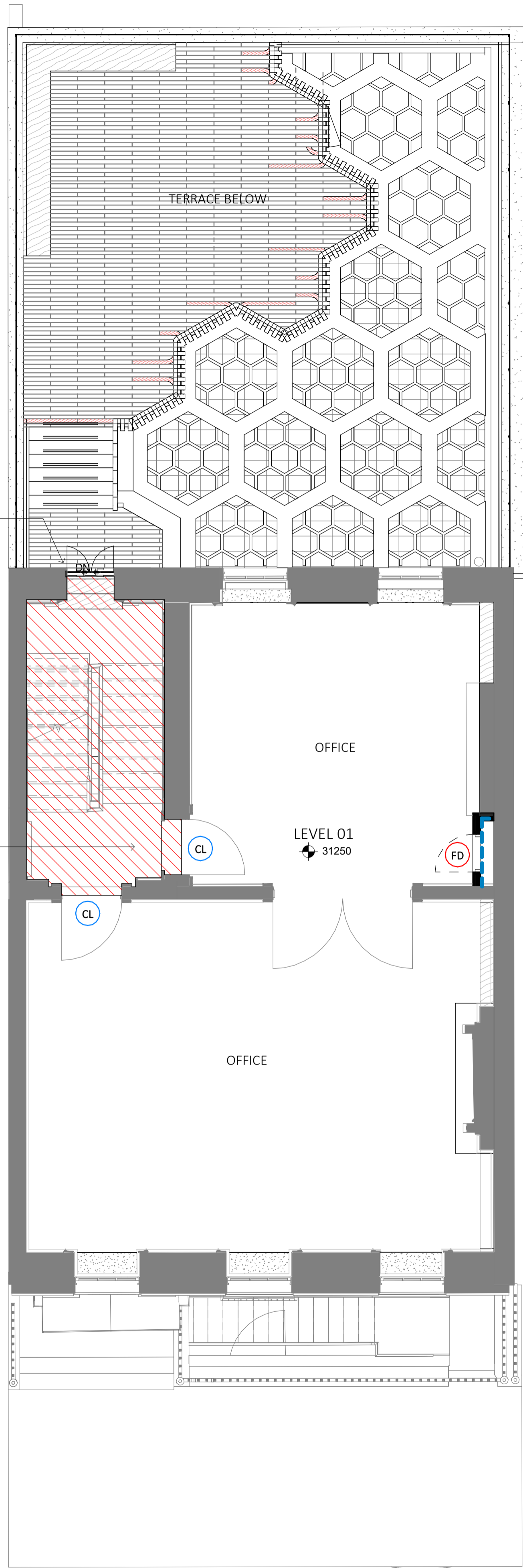
1 Proposed Level 01 - Fire Strategy 1 : 50
