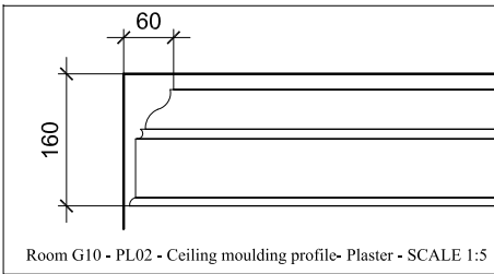
Room G10 - PL02 - Ceiling moulding profile- Plaster - SCALE 1:5
