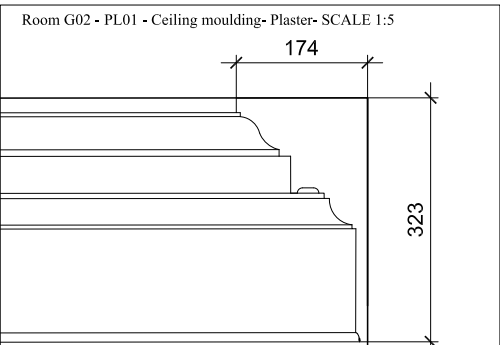
Room G02 - PL01 - Ceiling moulding- Plaster- SCALE 1:5
