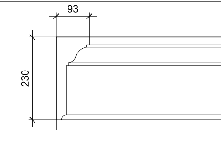
Room G06 - PL01 - Ceiling moulding profile- Plaster - SCALE 1:5
