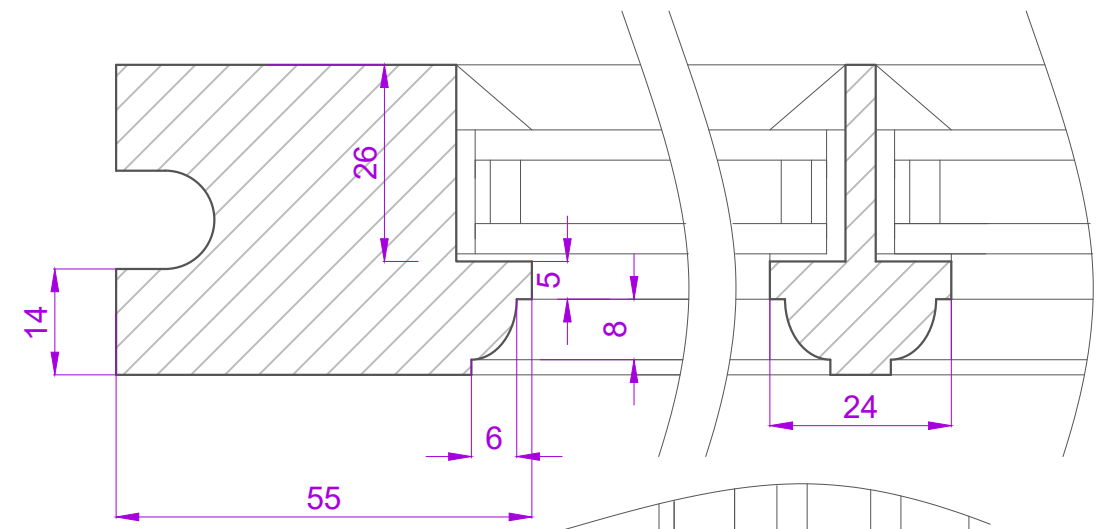
SECTION THROUGH STILE SCALE 1:1
