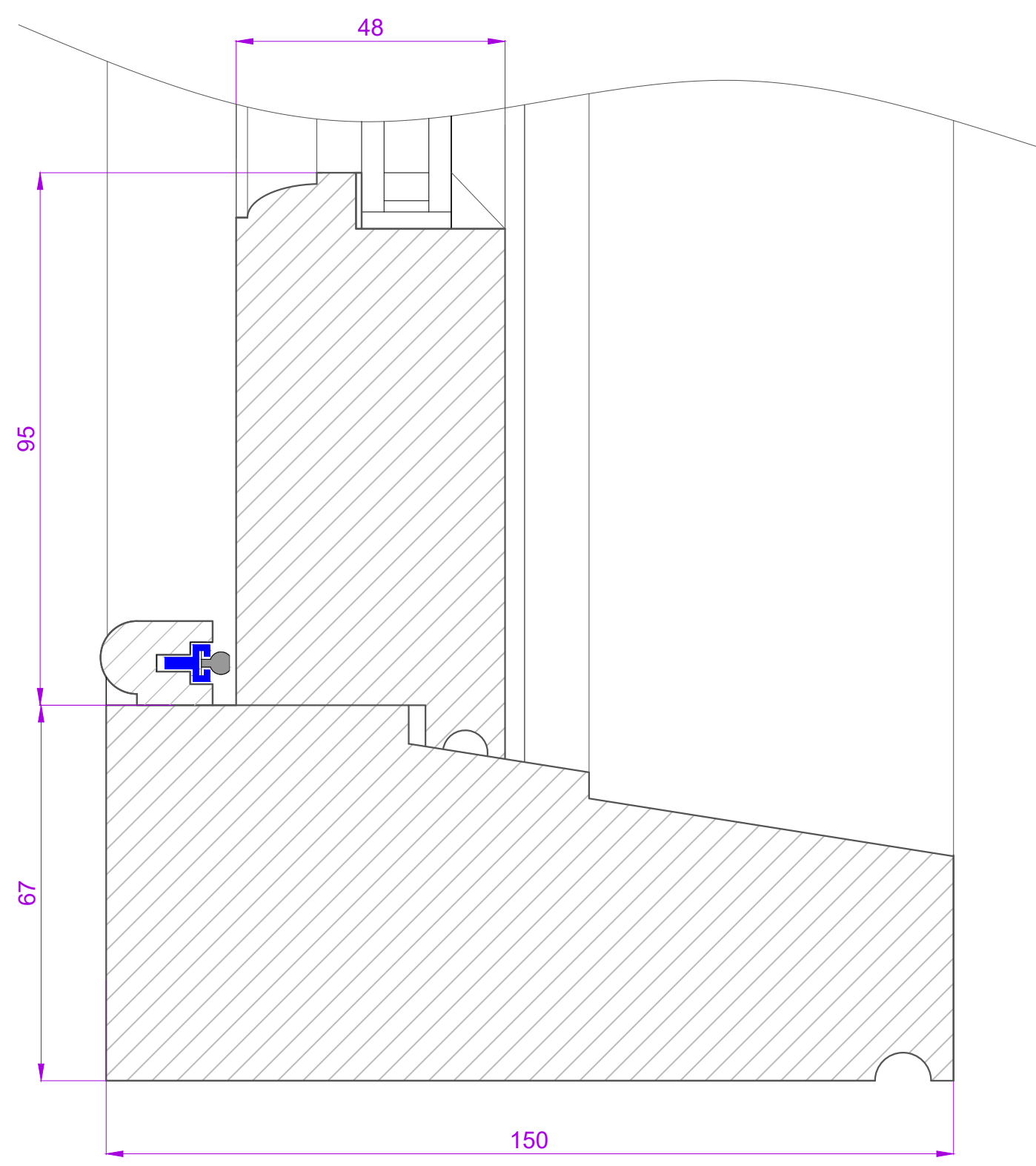
SECTION THROUGH CILL SCALE 1:1
