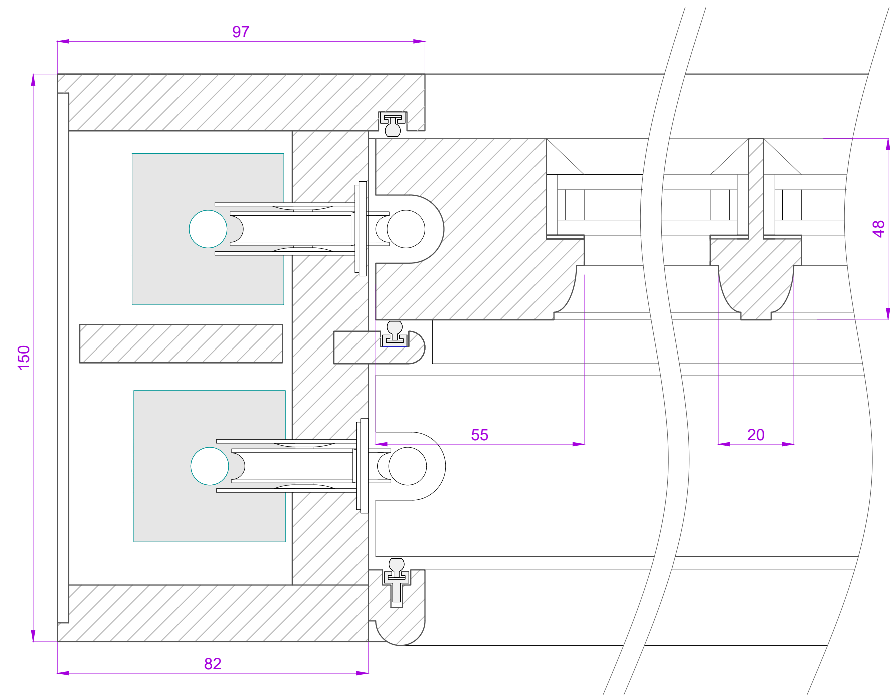
SECTION THROUGH FRAME JAMB SCALE 1:1
