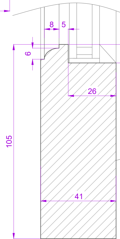
SECTION THROUGH CILL SCALE 1:1
