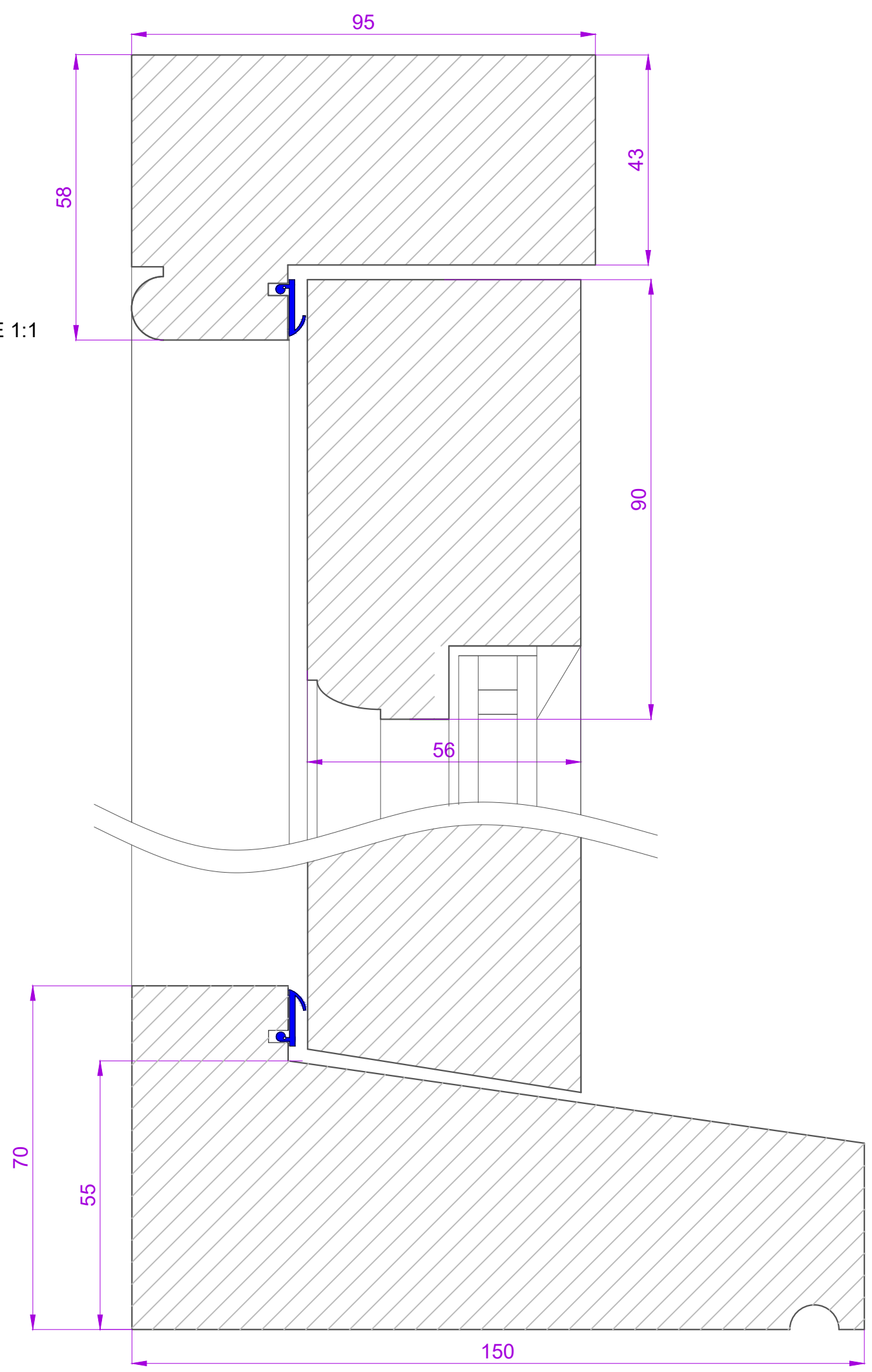
SECTION THROUGH CILL SCALE 1:1
