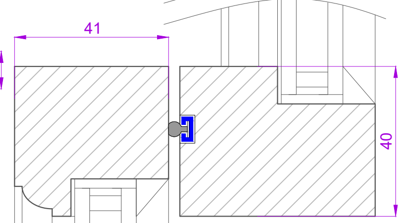
SECTION THROUGH MEETING RAIL SCALE 1:1
