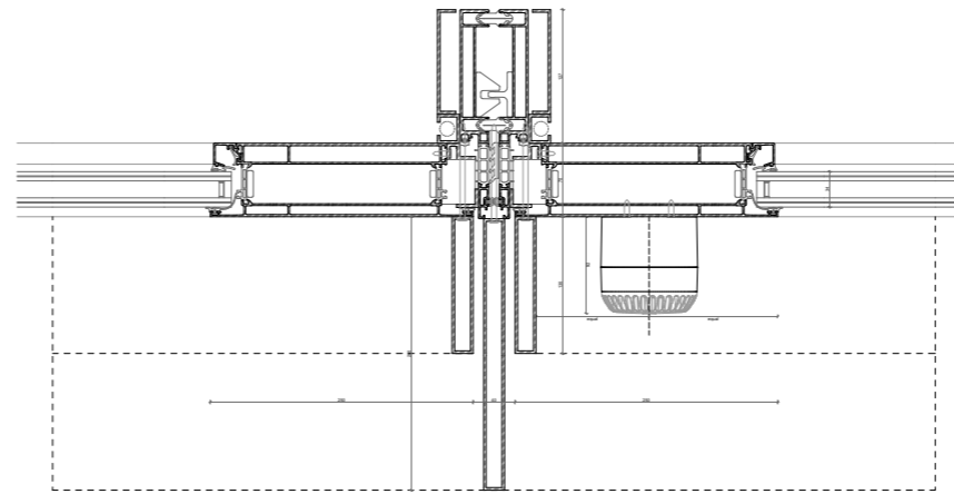
01 - Elevation - Visual beacon fixing location
