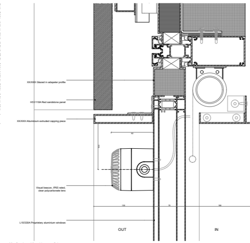
02 - Section - Visual beacon fixing
