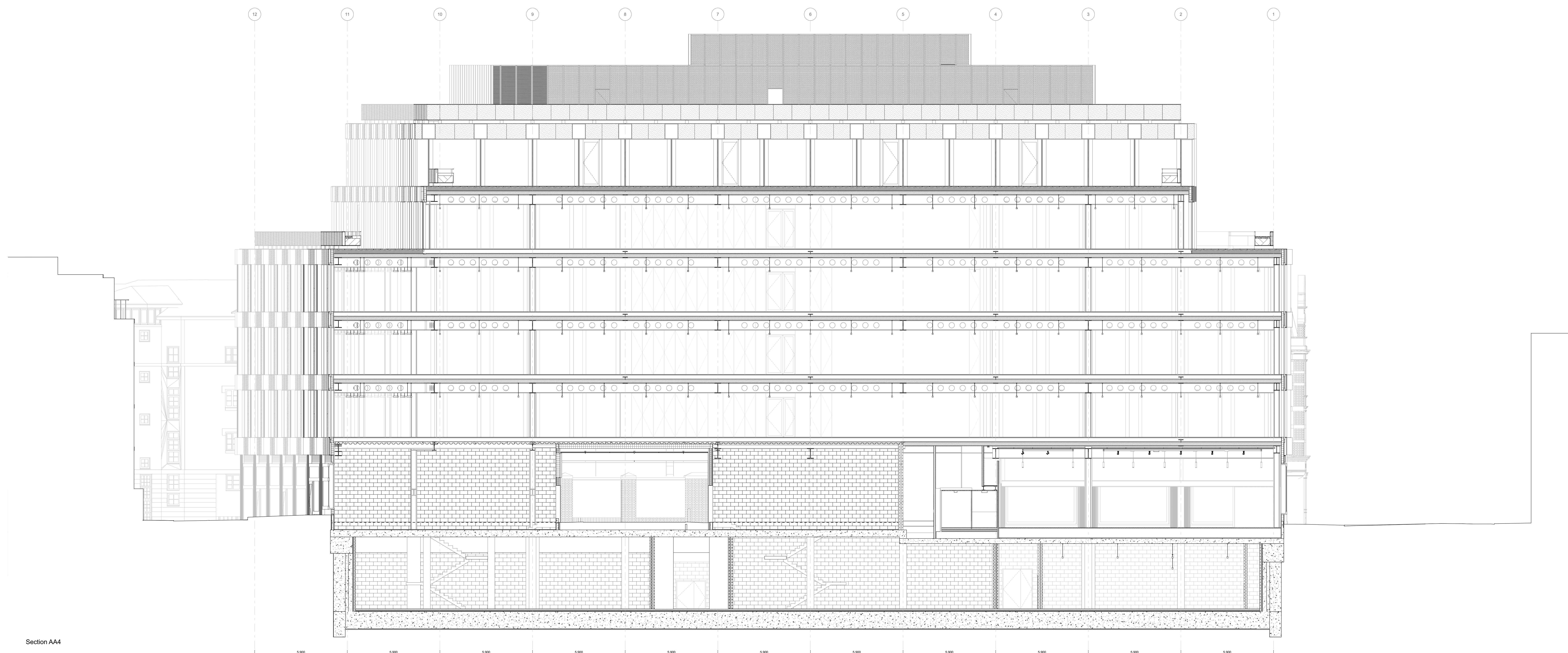
Section BB6
