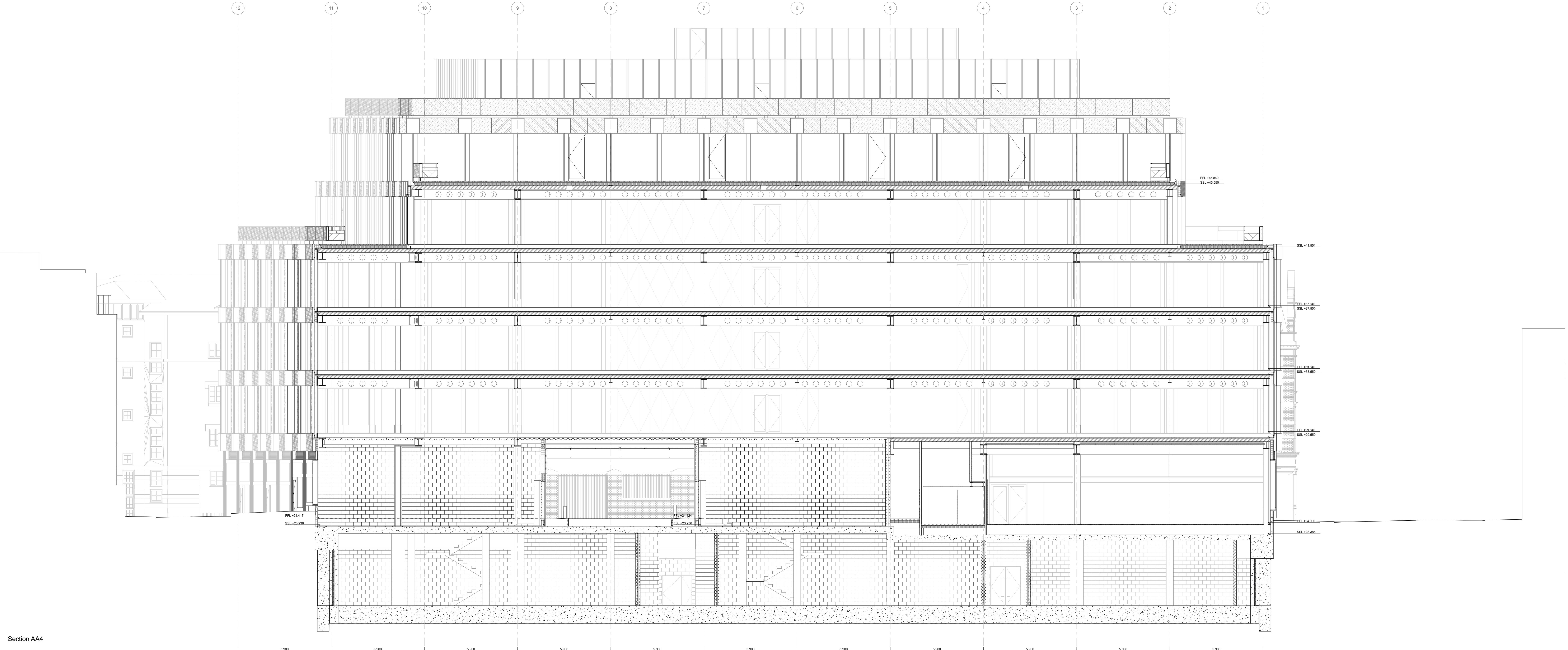
Section BB6
