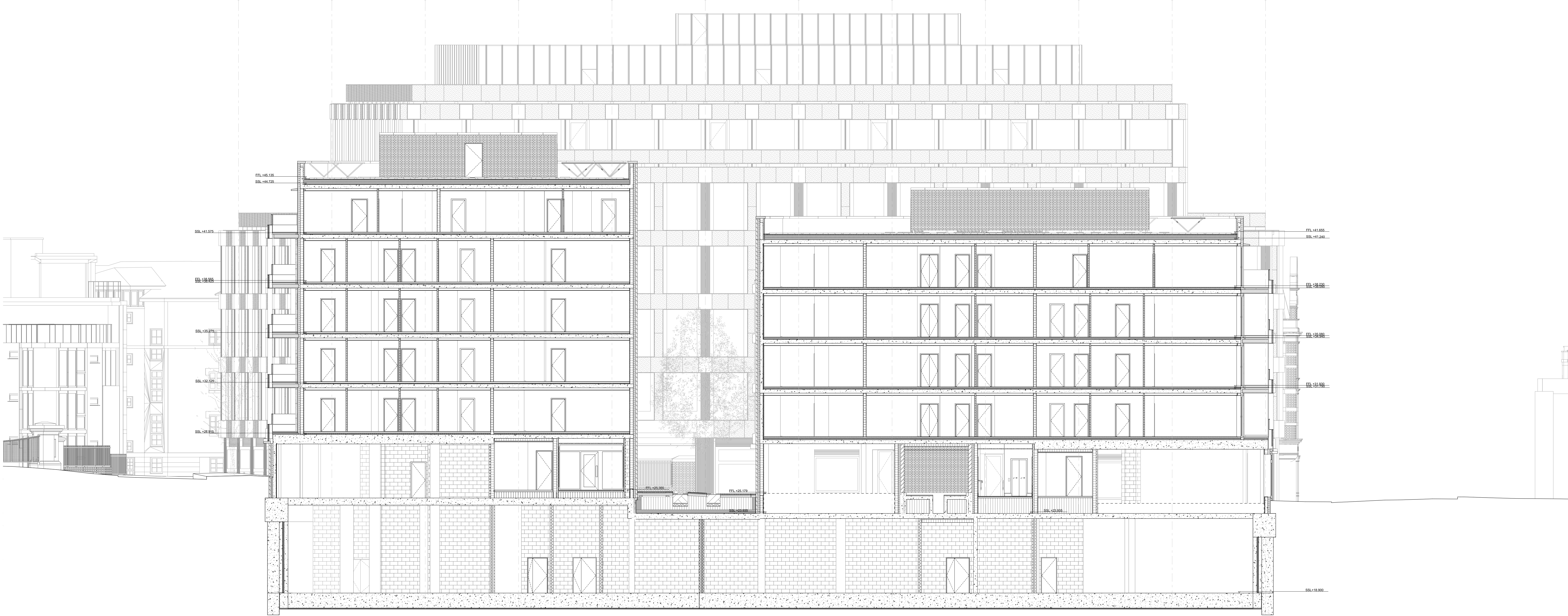
Section AA1
