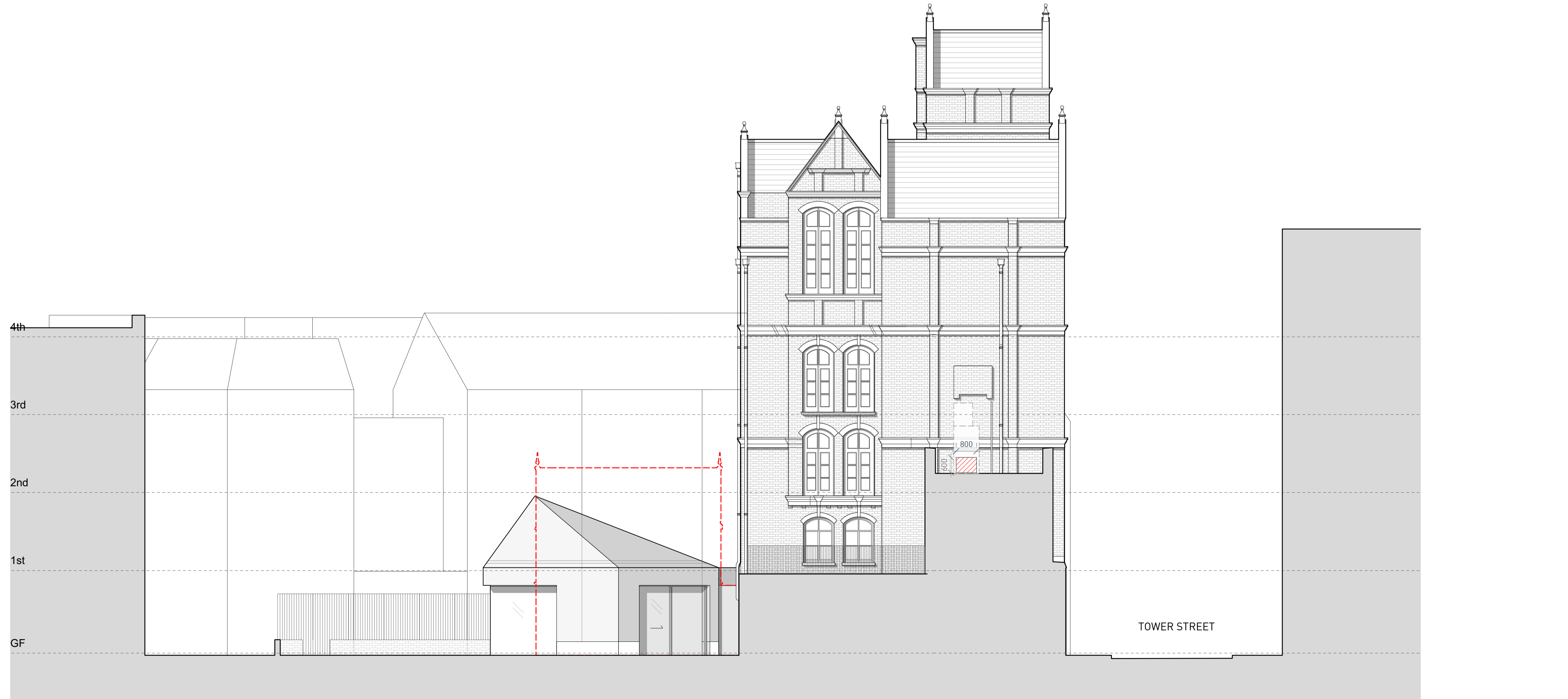
Side Elevation
