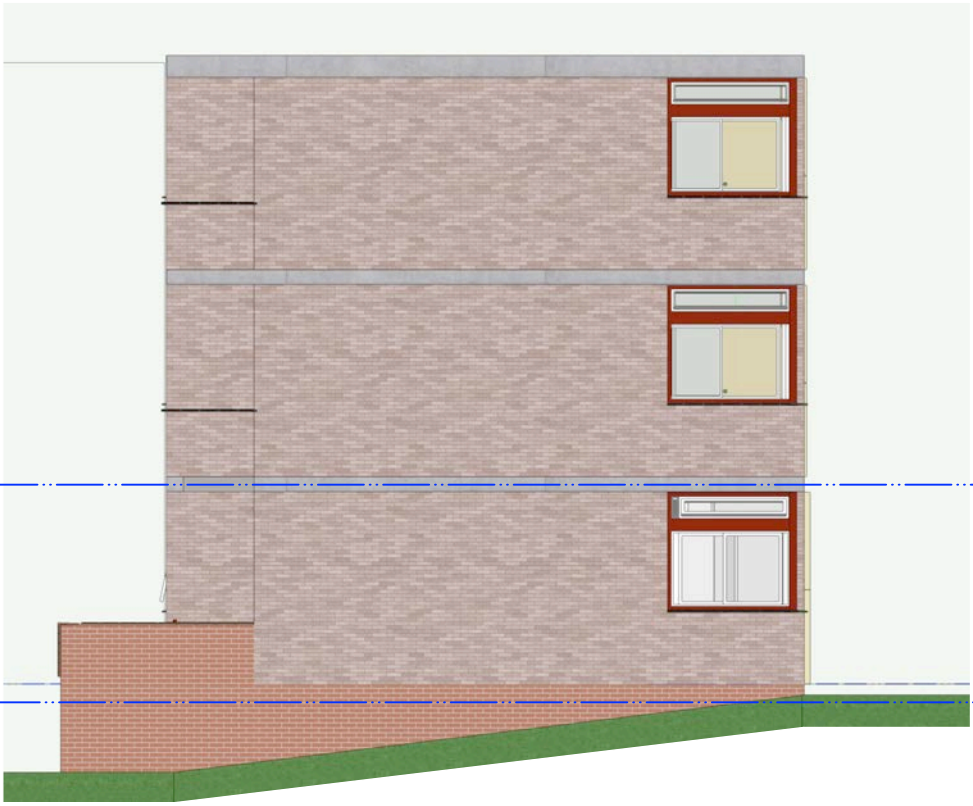
WEST ELEVATION
