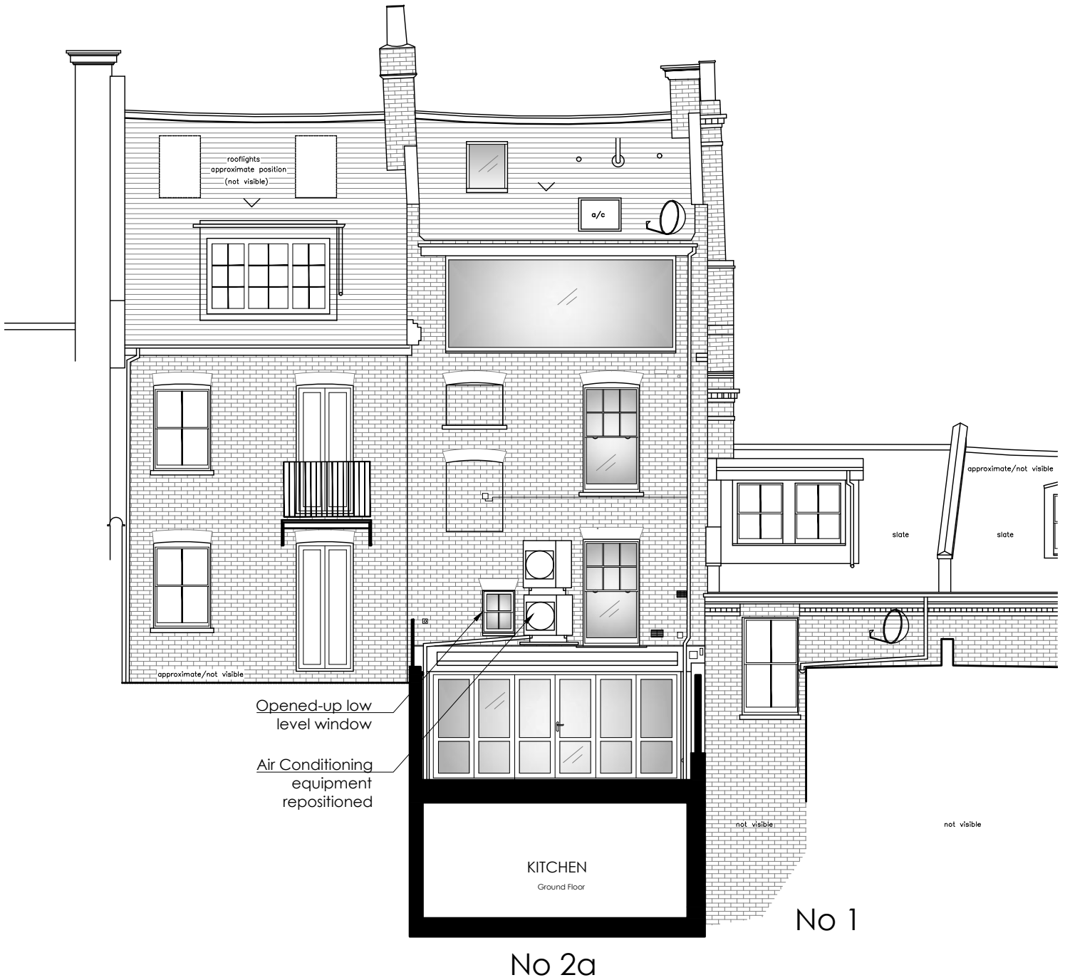
SOUTH EAST ELEVATION (Rear) ▲ 105.00m
