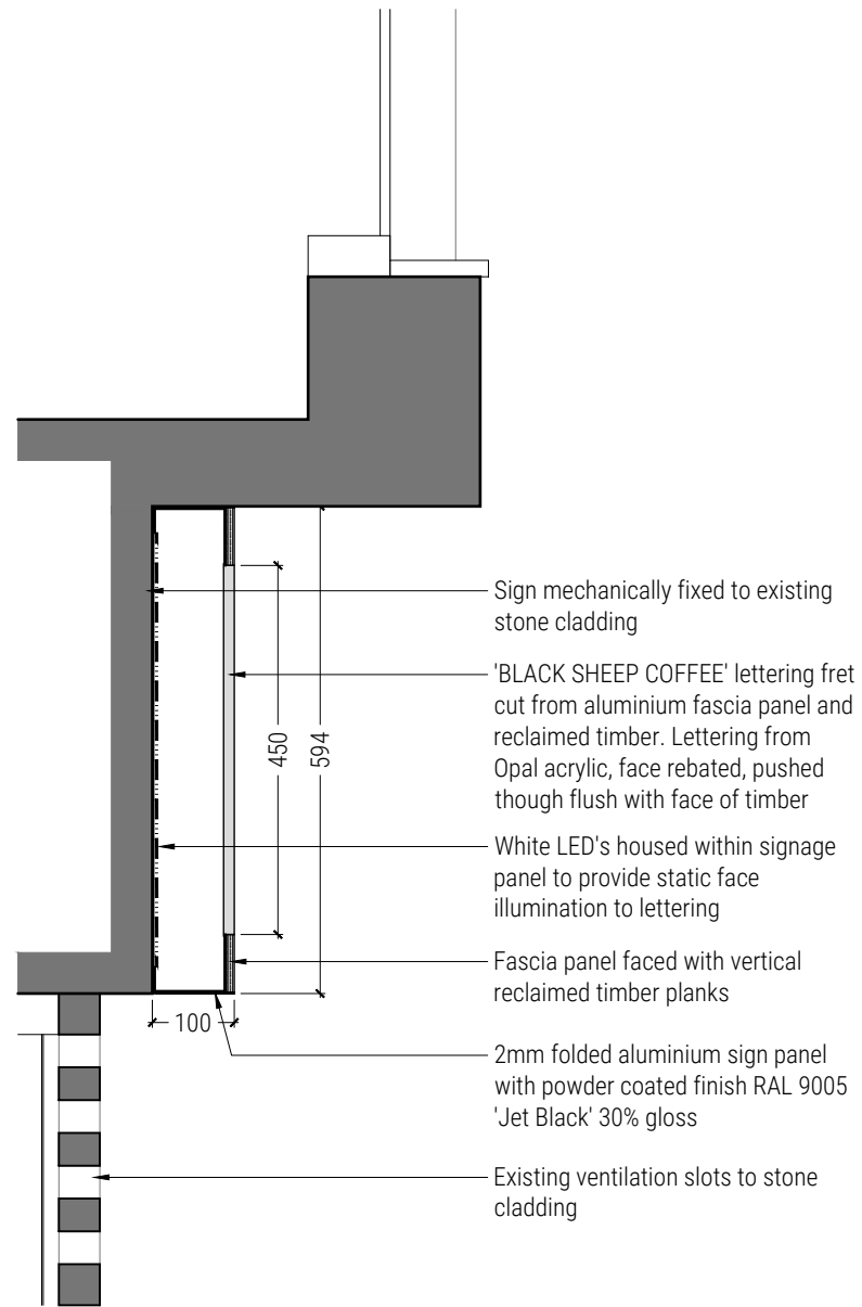
Section Through Fascia Sign
