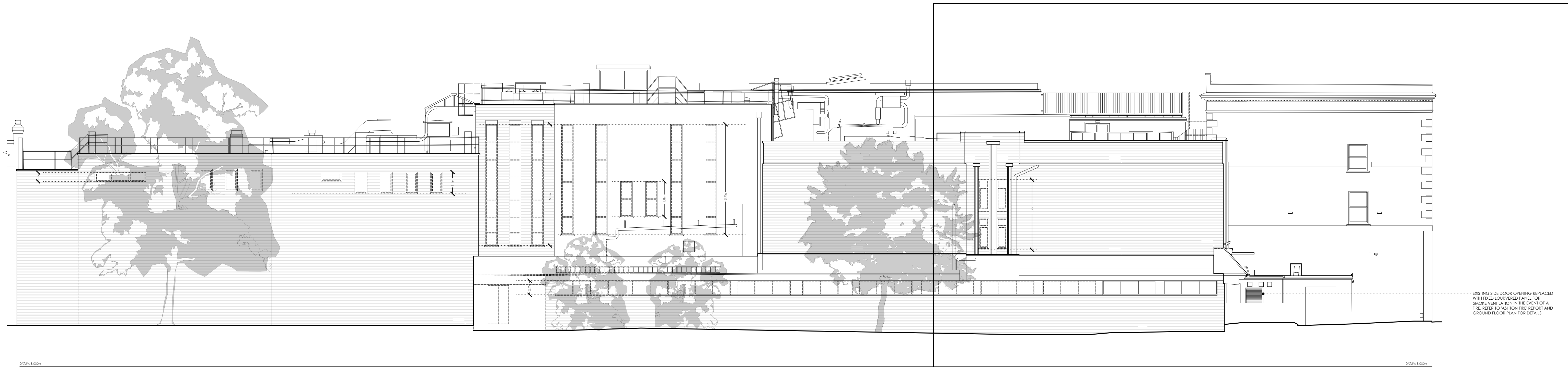
EAST ELEVATION
