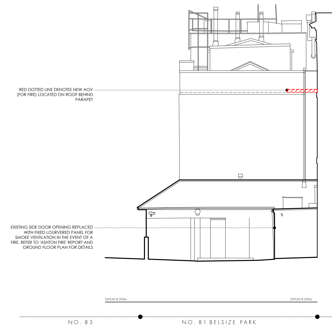
STREET ELEVATION
