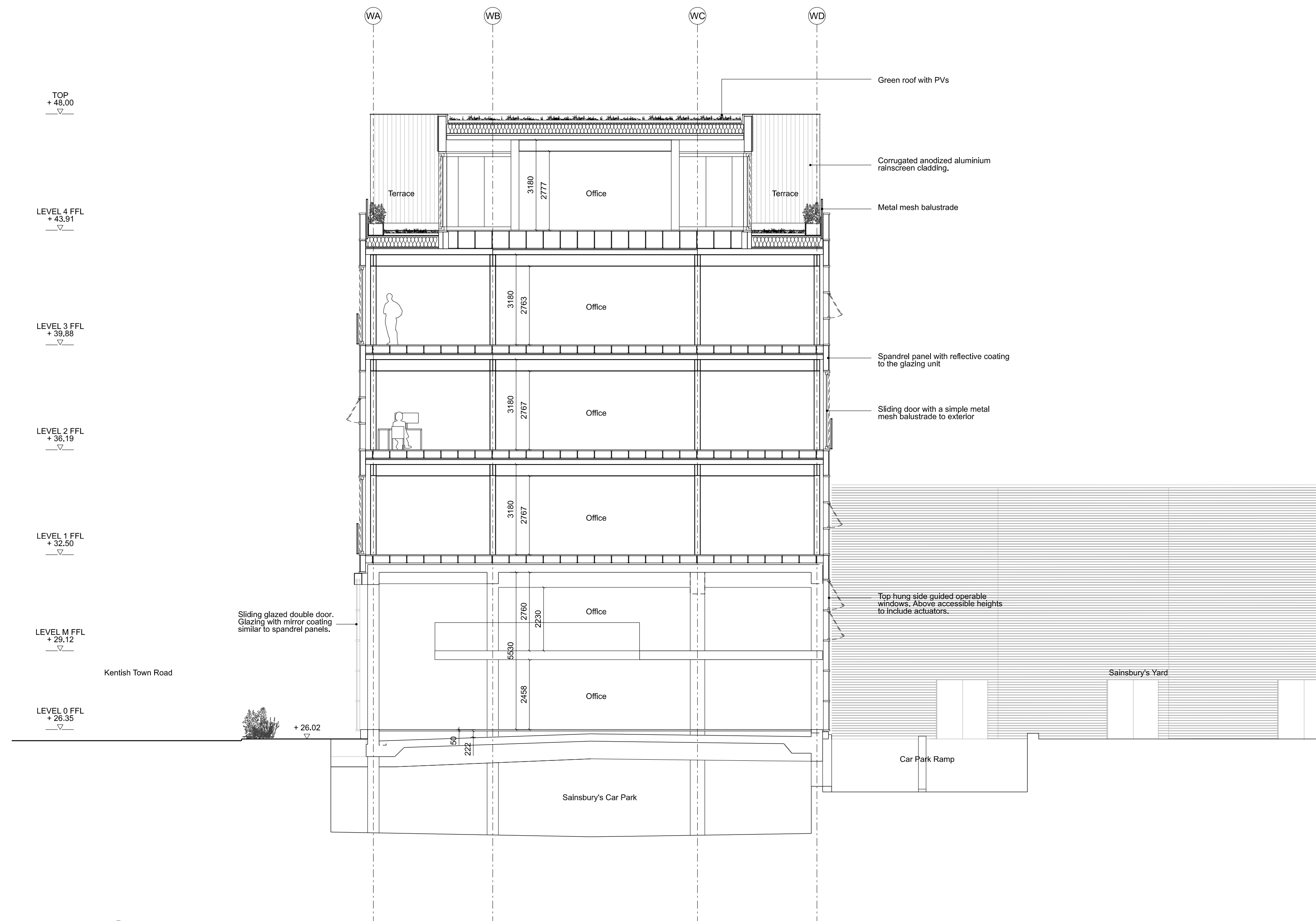
1 PROPOSED SECTION BB SCALE 1:200 @ A3
