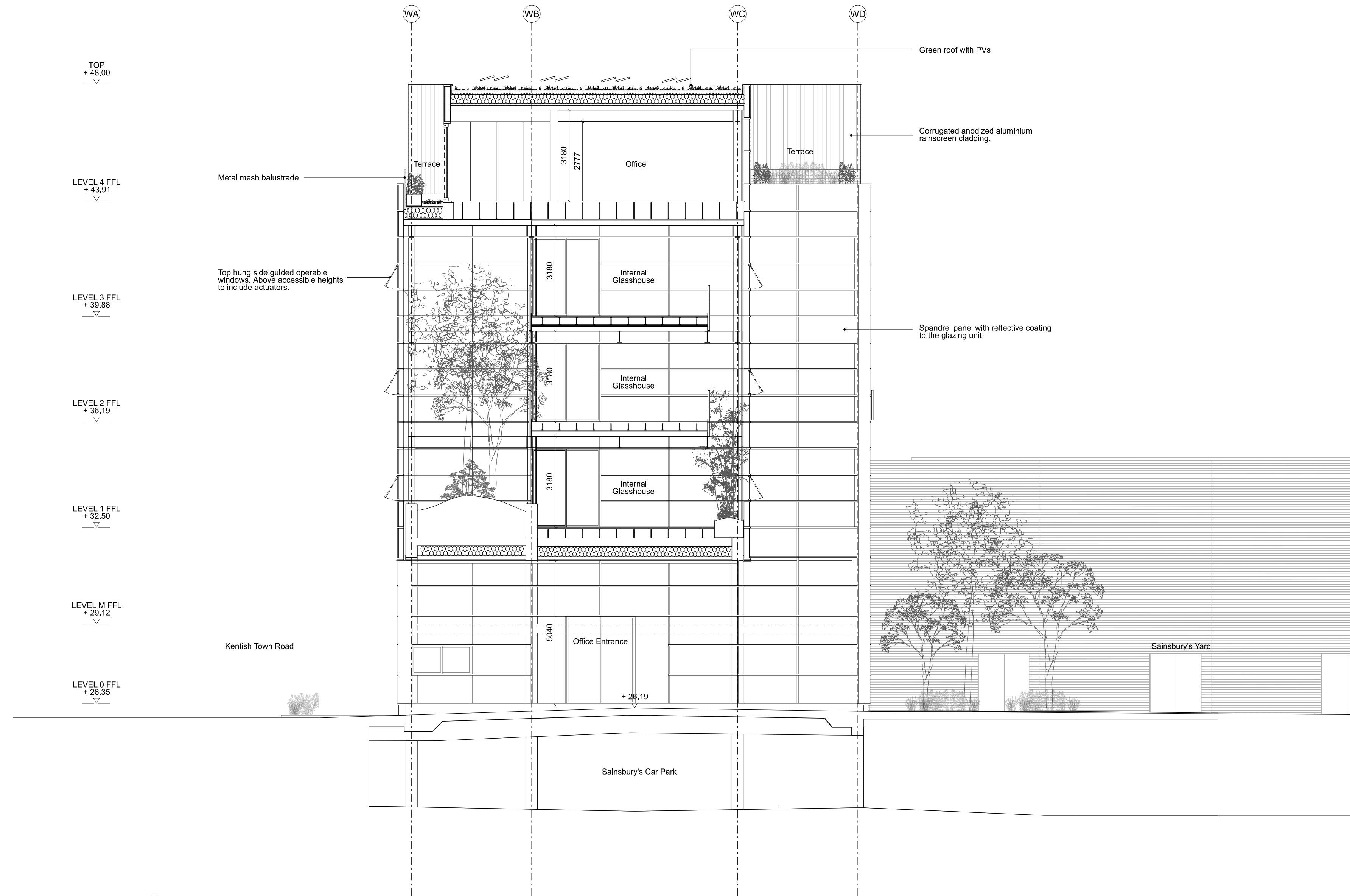
1 PROPOSED SECTION CC SCALE 1:200 @ A3
