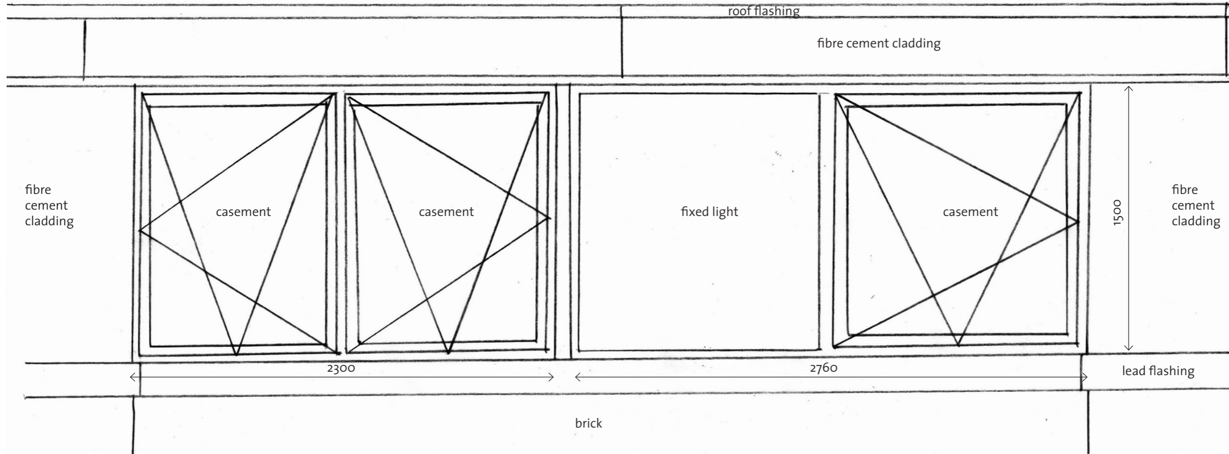
Existing upvc windows Inward opening side and bottom hung casements, white upvc frames, double glazed, sizes 2300 x 1500 and 2760 x 1500.
