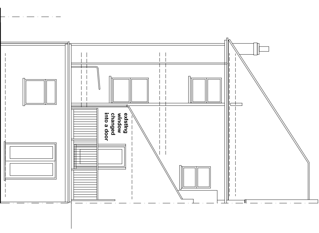
REAR ELEVATION AS PROPOSED
